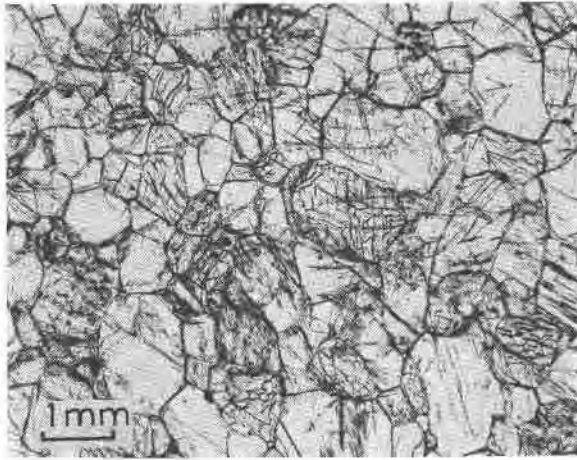
FIG. 3. Bronzitite from upper part of Transition Zone, Jagdlust. The rock averages 99.3 percent bronzite by volume. Apart from traces of alteration products, no other mineral is present in the area shown in the photograph. Plain light.
