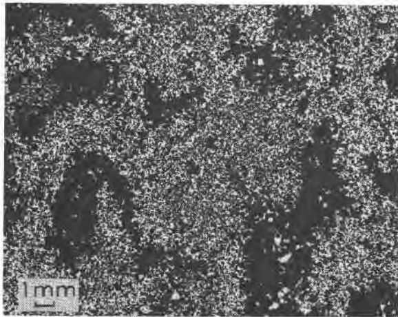
FIG. 7. Photomicrograph of thin chromitite seam in the L unit. Mottled black and white areas are bronzite and plagioclase crystals poikilitic with fine-grained chromite; the crystals are partly separated by coarser chromite (solid black). Central part of photograph is occupied by two poikilitic bronzite crystals. Other poikilitic crystals (e. g., along left side of photograph) are mostly plagioclase. Plain light, \times 5 .
