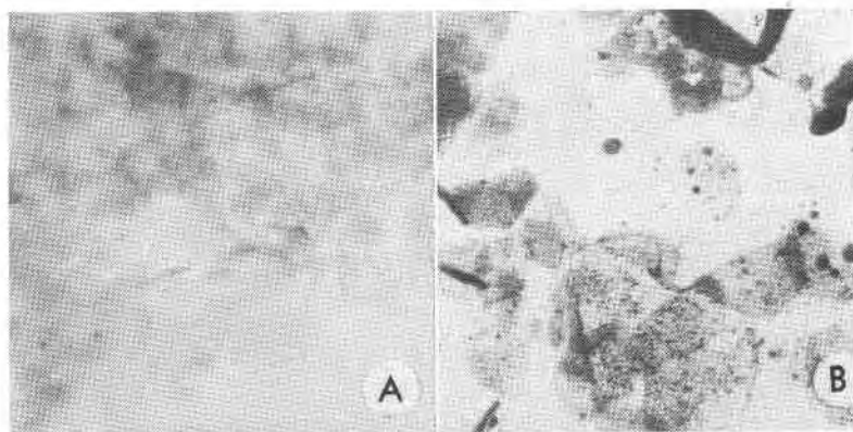
FIG. 3. Electron micrographs of sodium montmorillonite at pH 1 (A) exposure time 25 hours, (B) 72 hours after "neutralization." Adsorption time 5 minutes.
