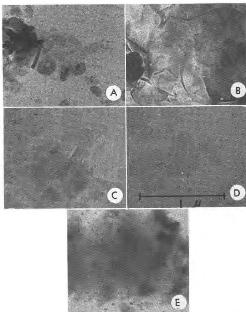
FIG. 1. Electron micrographs of sodium montmorillonite at (A) pH 1, (B) pH 4, (C) pH 6, (D) pH 11 and (E) pH 13. Adsorption time 5 minutes.
