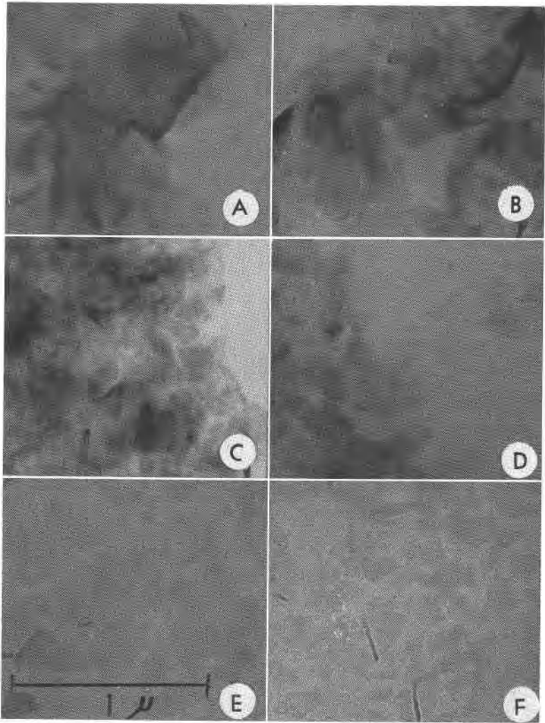
FIG. 2. Electron micrographs of sodium montmorillonite at various adsorption times, pH 4: (A) 5 minutes, (B) 10 minutes, (C) 20 minutes; pH 9, (D) 5 minutes, (E) 10 minutes, (F) 20 minutes.
