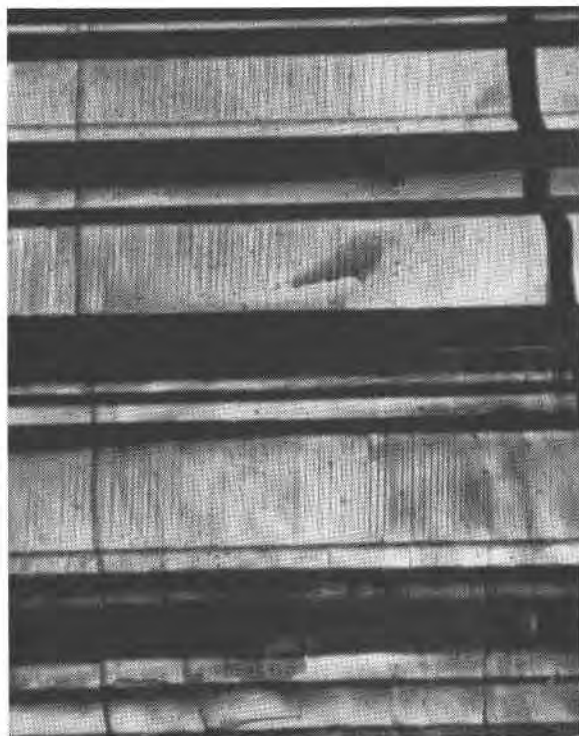
FIG. 2. Pericline inversion-twinning, developed in the high part.
