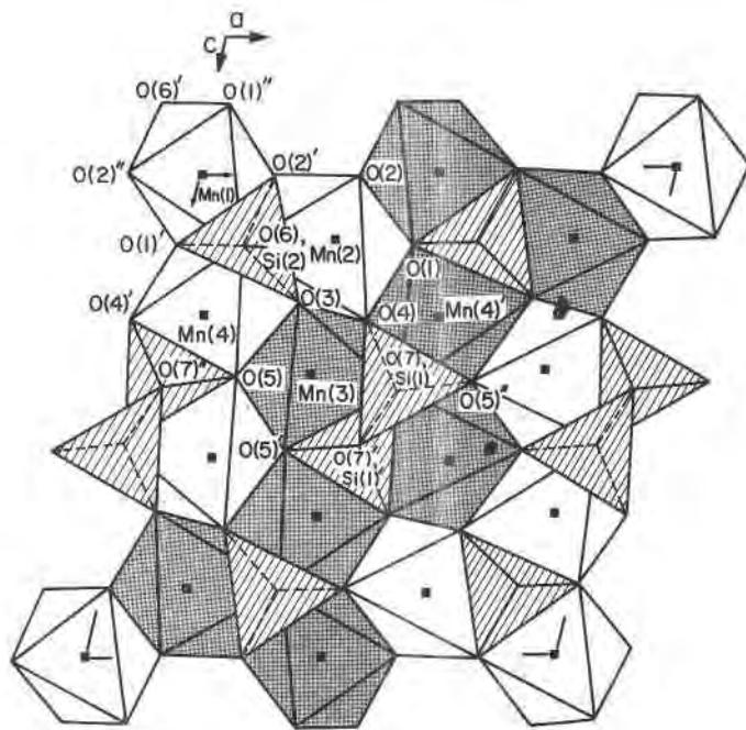
FIG. 1. Polyhedral diagram of the leucophoenicite crystal structure, projected down the y -axis. The atomic species are labelled in conformity with the text: unprimed labels are the atomic positions in Table 4 and primed labels are their symmetry equivalents. Silicon atoms reside in the centers of the ruled tetrahedra. Unshaded octahedra are at y \sim 0 , stippled octahedra at y \sim 1/2 .
