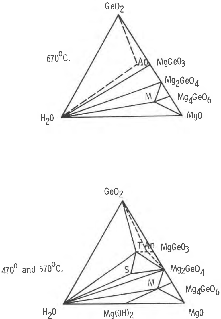
FIG. 2. Equilibrium relations in the system \text{MgO-GeO}_2\text{-H}_2\text{O} . ( \text{M} = \text{Mg}_2\text{GeO}_4 \cdot \text{Mg(OH)}_2 )
