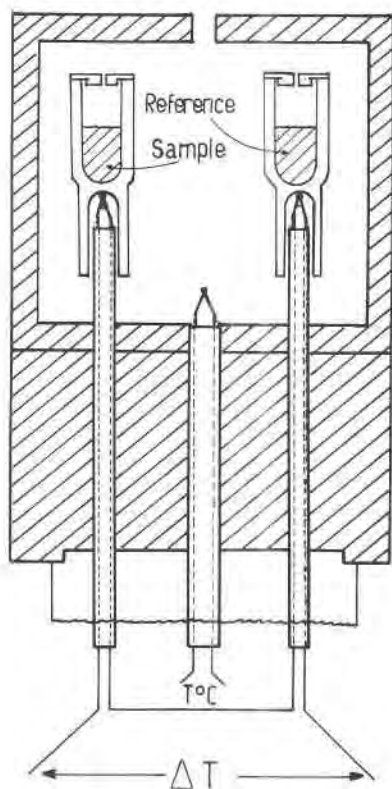
FIG. 2. Measuring head for DDC.
