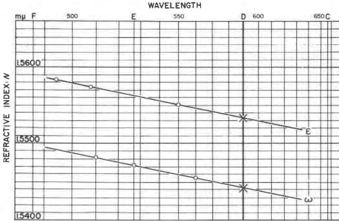
Fig. 1. Hartman net graph of quartz standard presented in the five step summary. This illustrates the agreement of orientation variation data and double variation data (X=orientation variation data and O=double variation data).
