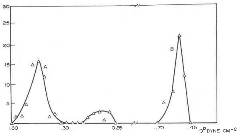
FIG. 1. Distribution curves of the Young's modulus of muscovite in the basal plane (the ordinate represents the frequency of observation and the abscissi represents the values of Young's modulus).
