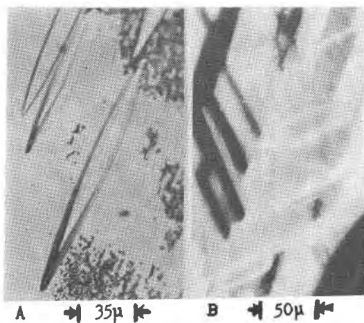
FIG. 2. Etch pits on the cleavage face of calcite crystals immersed in \text{NH}_4\text{F} . A. Crystal etched 1 hour in 0.5 F \text{NH}_4\text{F} with surface fluorite layer removed to reveal the deepening of the "prow" of the boat-shaped pit and the development of a right angle in the lower pit. B. Crystal etched 10 days in 0.1 F \text{NH}_4\text{F} with transformed layer removed to show well-formed hexagonal pits.
