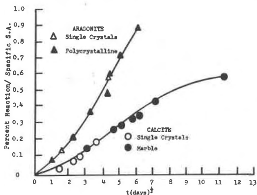
FIG. 8. The effect of surface area on the rate of reaction of calcite and aragonite with 1.0 F \text{NH}_4\text{F} .
