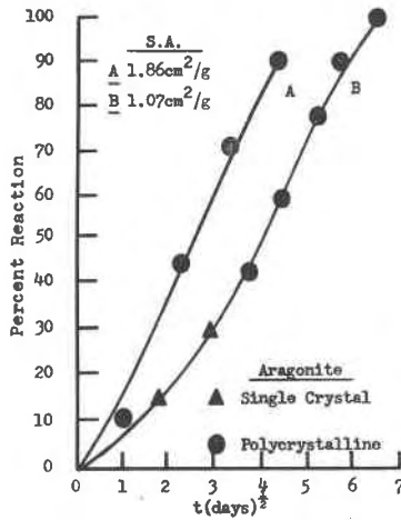
FIG. 5. The rates of reaction of aragonite specimens with 1.0 F \text{NH}_4\text{F} .
