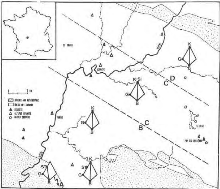
FIG. 1. The disposition of the various mineralogical zonation units found are indicated on the sketch map of the area studied. The assemblages have been projected on an A-F-M surface, after the method proposed by Thompson (1957). The assumptions which permit the use of this projection, the presence of muscovite and quartz in all facies, are generally fulfilled in the rocks under investigation.
