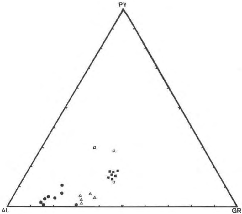
FIG. 4. Estimated compositions of garnets (Winchell, 1958) from four types of rocks in the Uzerche area are shown on pyrope-almandine-grossular coordinates. Chemical compositions of three garnets show the method to underestimate the pyrope molecule content by about 10 percent.
