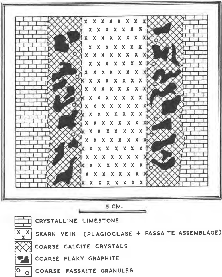
FIG. 1. Sketch of Calc-silicate skarn vein near Gondivalasa.
