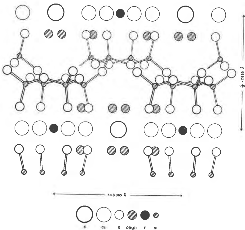
FIG. 3. The structure of apophyllite projected on (100).
