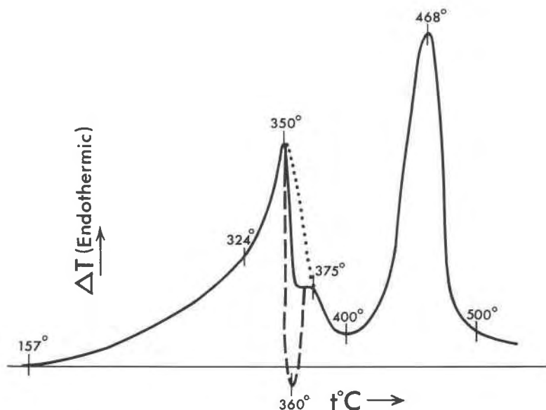
FIG. 4. Differential thermal analysis curve of apophyllite from Mont. St. Hilaire, Quebec. The theoretical curve, in the absence of ordering of \text{H}_2\text{O} , is represented by the dotted line and the theoretical exothermic peak, due to ordering of \text{H}_2\text{O} , is represented by the dashed line.
