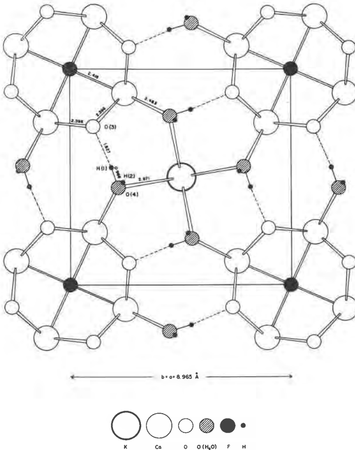
FIG. 2. The K, Ca sheet in apophyllite projected on (001).
