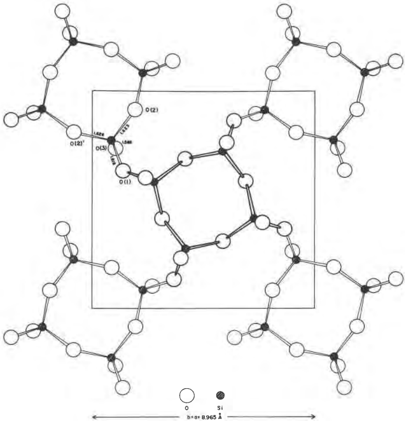
FIG. 1. The \text{Si}_8\text{O}_{20} sheet in apophyllite projected on (001).
