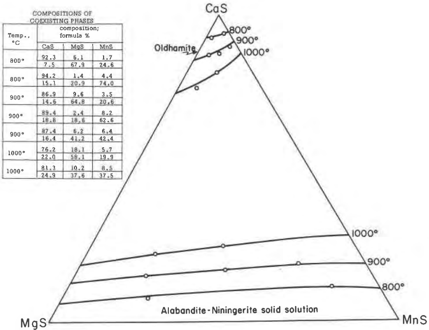
FIG. 12. The ternary solvus in the system CaS-MgS-MnS. Compositions of coexisting phases were determined by microprobe analysis.
