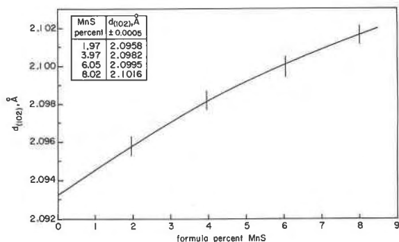
FIG. 4. The effect of Mn replacing Fe in troilite, shown by an increase in the spacing of the (102) reflection of the troilite sub-cell.
