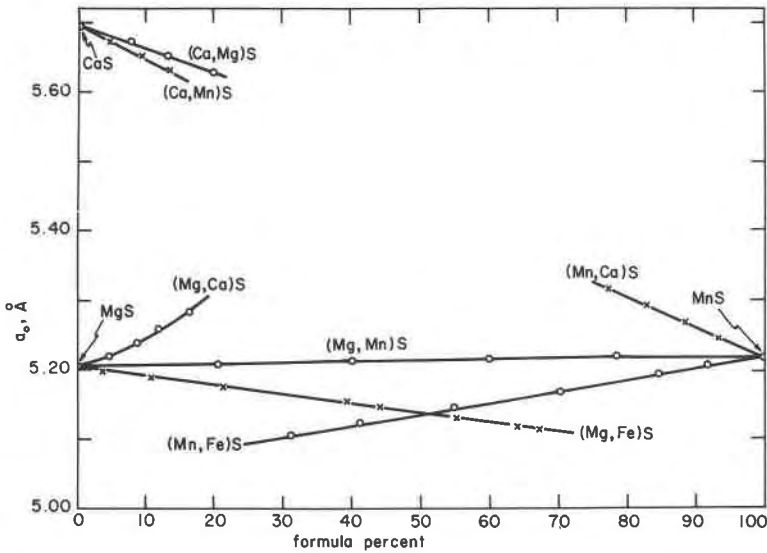
FIG. 2. Effect of binary cation substitutions on the unit cell edges of cubic monosulfide solid solutions. Data are given in Table 2.
