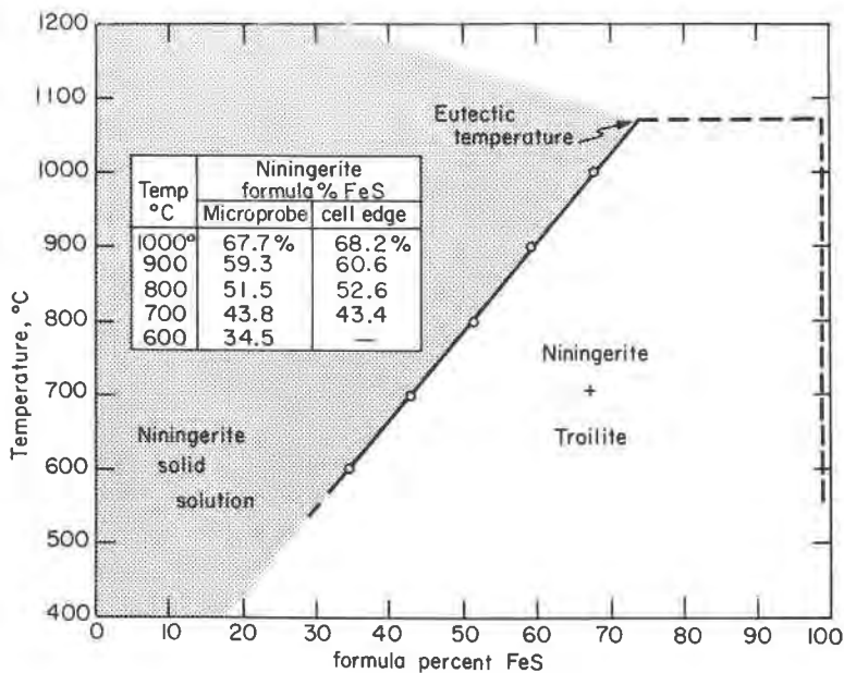
FIG. 6. The solvus between niningerite and troilite.
