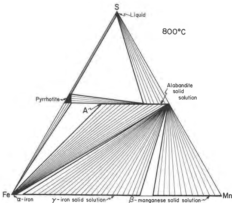
FIG. 1. Phase diagram for the system Fe-Mn-S at 800°C. The extensive alabandite solid solution coexists with \alpha -iron, reaching a maximum at point A where it coexists with manganiferous troilite and \alpha -iron.
