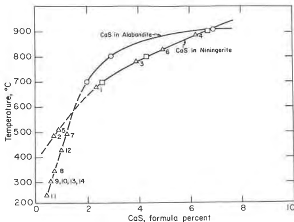
FIG. 14. The CaS-contents of alabandites and niningerites coexisting with oldhamite and troilite. Numbered points refer to meteorite samples (after Keil, 1968), listed in Table 6.
