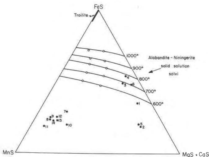
FIG. 13. Compositions of niningerites and alabandites from enstatite chondrites (after Keil, 1968), normalized to MgS, MnS, CaS, FeS, and with CaS plotted as MgS, plotted on the ternary solvus in the system FeS-MgS-MnS. Minimum temperatures of formation can be read directly from the diagram. Specimen numbers refer to samples listed in Table 2.
