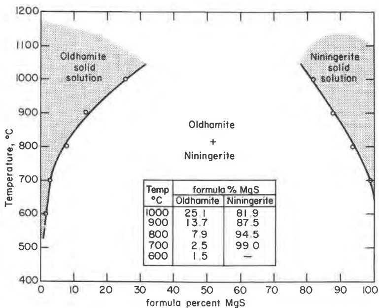
FIG. 8. The solvus between oldhamite and niningerite. Phase compositions were determined from unit cell edge measurements.
