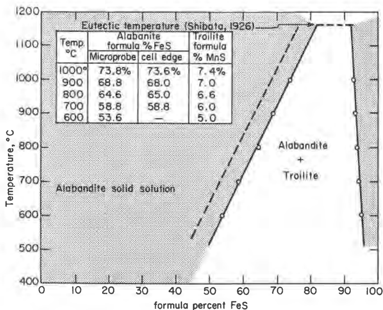
FIG. 5. The solvus between alabandite and troilite. The dashed line is the solvus determined by Shibata (1926) using "appearance of phase" runs. There is a question regarding the accuracy of Shibata's temperature measurements (see text).
