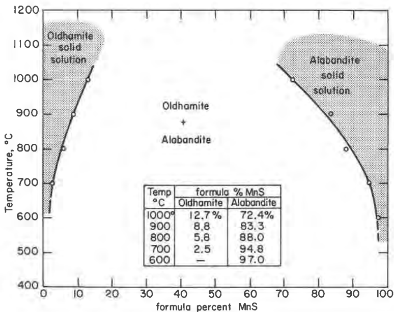
FIG. 7. The solvus between oldhamite and alabandite. Phase compositions were determined from unit cell edge measurements.
