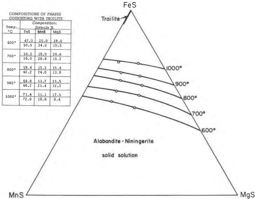
FIG. 9. The ternary solvus in the system FeS-MnS-MgS. Phase compositions were determined by microprobe analysis.
