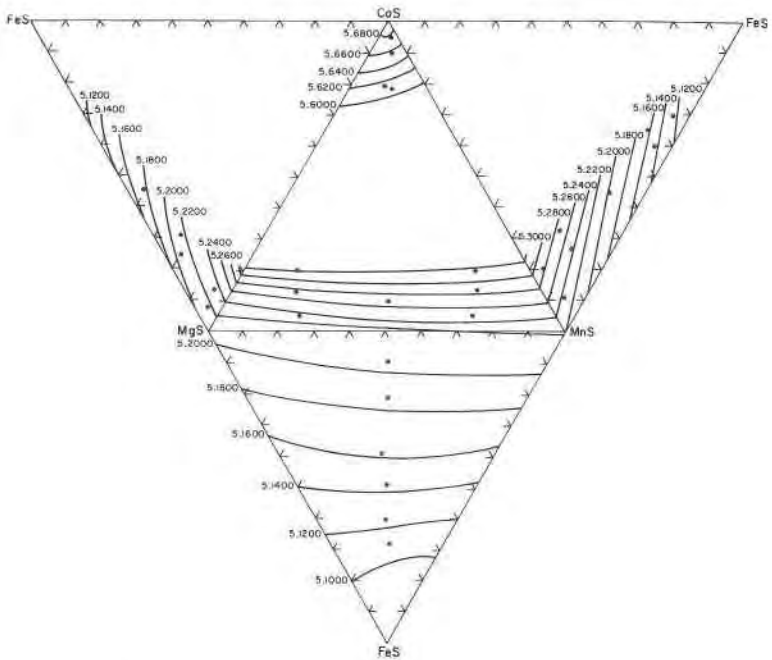
FIG. 3. Effect of ternary cation substitutions on the unit cell edges of cubic monosulfide solid solutions. Data are given in Table 3.
