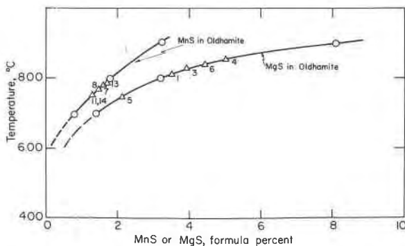
FIG. 15. The MnS-, and MgS-contents of oldhamite coexisting with troilite and alabandite or niningerite respectively. Numbered points refer to meteorite samples (after Keil, 1968), listed in Table 6.
