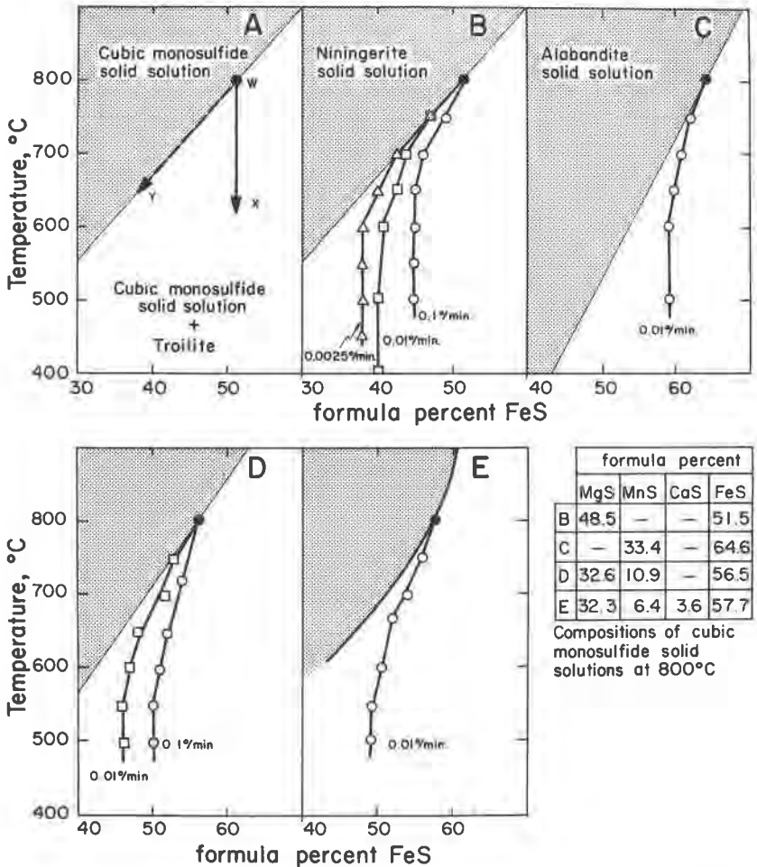
FIG. 16. Composition changes in cubic monosulfide solid solutions cooled at different rates. Solid solutions were equilibrated with troilite for three months, cooled at fixed rates and samples withdrawn at specific temperature intervals. Compositions were determined by unit cell measurements.
