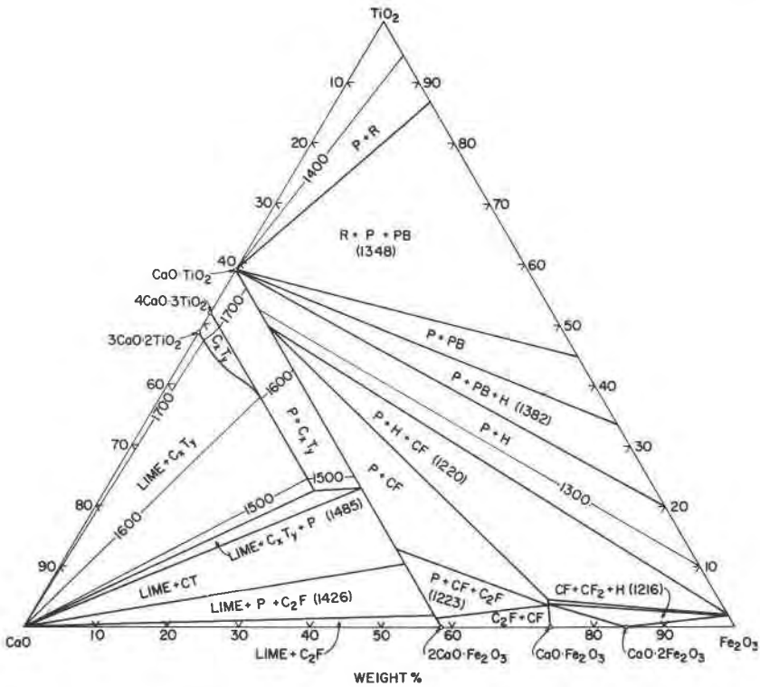
FIG. 6. Solidus surface of the system CaO-iron oxide-TiO 2 in air. Light lines are solidus isotherms drawn at 100°C intervals. Numbers in parentheses are solidus temperatures within composition triangles where three crystalline phases coexist with liquid. Boundary curves outlining the region of Ca 4 Ti 3 O 10 -Ca 3 Ti 2 O 7 solid solutions are dashed because of the uncertainties still existing regarding the nature of this phase. Abbreviation used in addition to those explained previously has the following meaning: P=perovskite.
