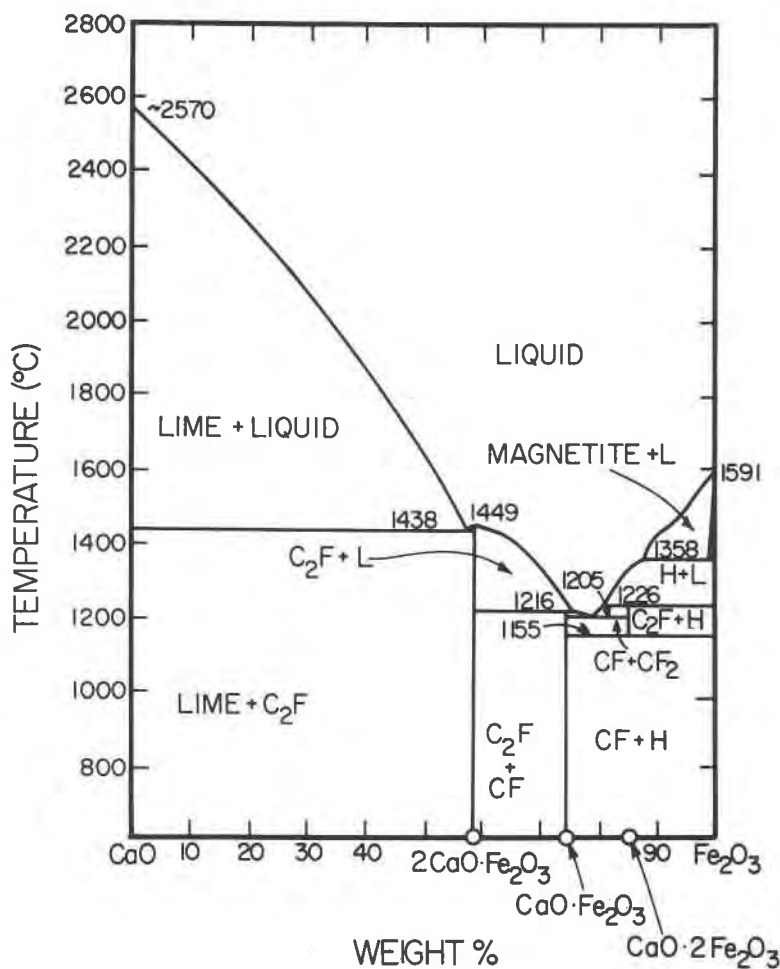
FIG. 2. Phase diagram for the system CaO-iron oxide in air, after Phillips and Muan (1958). Abbreviations used have the following meanings: C 2 F = dicalciumferrite (Ca 2 Fe 2 O 5 ); CF = monocalciumferrite (CaFe 2 O 4 ); CF 2 = monocalciumdiferrite (CaFe 4 O 7 ); H = hematite; L = liquid.
