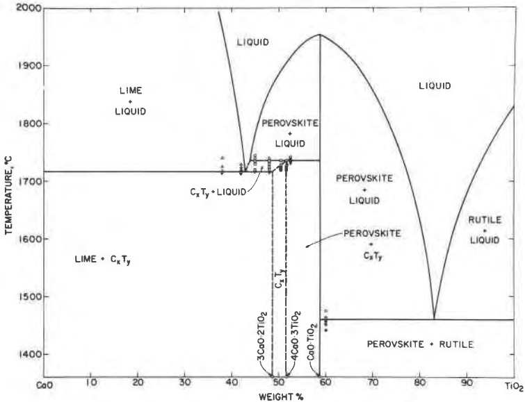
FIG. 4. Suggested revised phase diagram for the system \text{CaO-TiO}_2 . Liquidus curves are mainly after DeVries, Roy and Osborn (1954), with tentative modifications of the diagram in the 4\text{CaO}\cdot 3\text{TiO}_2-3\text{CaO}\cdot 2\text{TiO}_2 composition range based on data obtained in the present investigation. The boundary curves in this region have been dashed because of the uncertainties still existing regarding each phase assemblage, as labelled on the diagram. Abbreviation used has the following meaning: C_xT_y = \text{Ca}_4\text{Ti}_3\text{O}_{10}-\text{Ca}_3\text{Ti}_2\text{O}_7 solid solutions.
