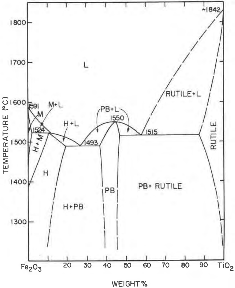
FIG. 3. Phase diagram for the system iron oxide-TiO 2 in air, after MacChesney and Muan (1959). Abbreviations used have the following meanings: M = magnetite; H = hematite; PB = pseudobrookite; L = liquid
