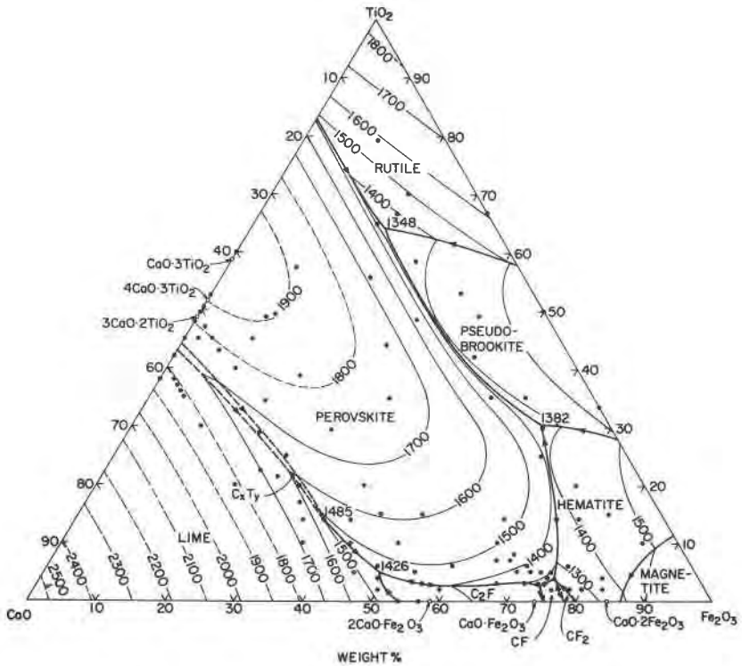
FIG. 5. Liquidus surface of the system CaO-iron oxide-TiO 2 in air. Solid dots represent compositions of mixtures studied. Liquidus isotherms are drawn at 100°C intervals. Boundary curves outlining the region of Ca 4 Ti 3 O 10 -Ca 3 Ti 2 O 7 solid solutions are dashed because of the uncertainties still existing regarding the nature of this phase. Abbreviations used have the same meanings as explained in legends to Figs. 2 and 4.
