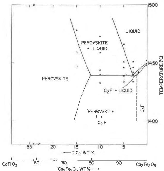
FIG. 7. Phase relations along the join CaTiO 3 -Ca 2 Fe 2 O 5 of the system CaO-iron oxide-TiO 2 in air. Dashed curves are inferred only. A different point symbol is used for each phase assemblage, as labelled on the diagram.
