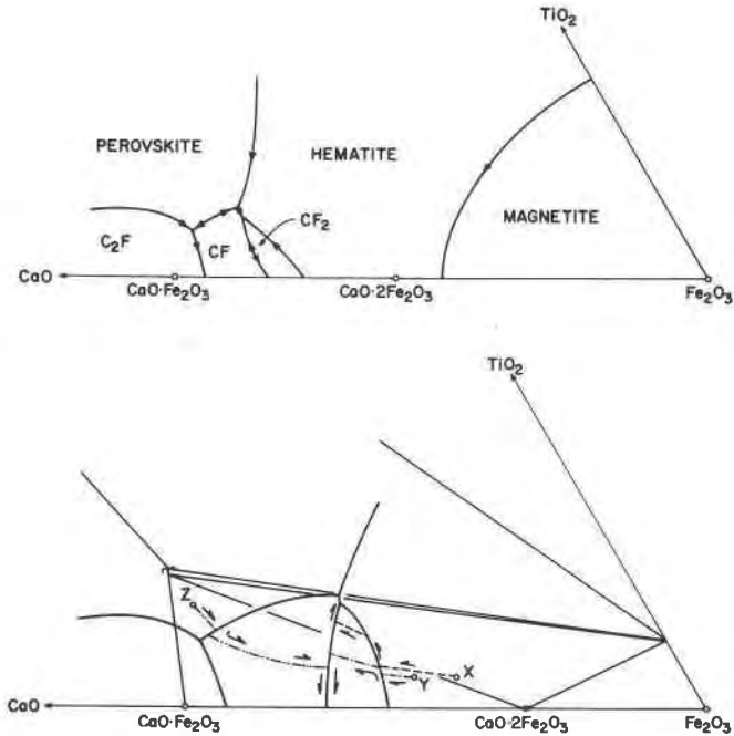
FIG. 8. Phase relations in the vicinity of the calcium ferrite areas of the liquidus surface of the system CaO-iron oxide-TiO 2 in air. An undistorted diagram is shown at the top, and a distorted diagram is presented below in order to better illustrate crystallization sequences of selected mixtures. In the latter diagram, the changes in liquid compositions of mixtures X, Y, and Z during equilibrium cooling are illustrated with arrows indicating directions of composition changes with decreasing temperatures.
