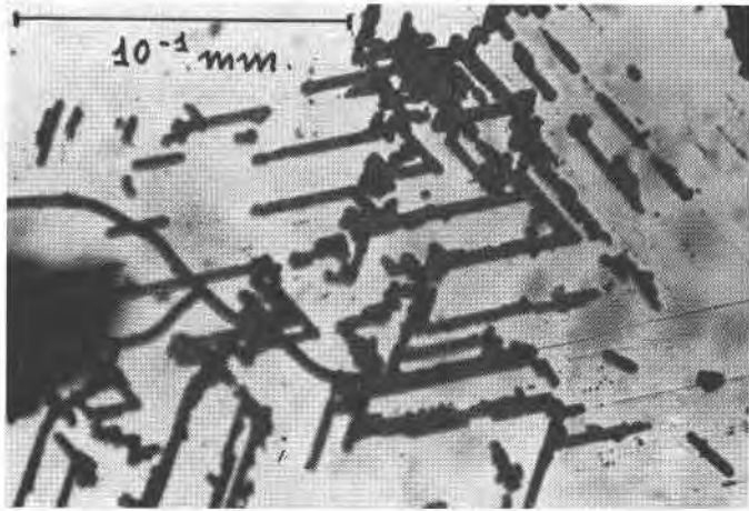
FIG. 1. Framework of goethite on hematite platelets.
