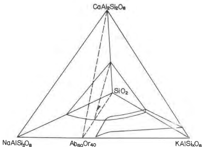
FIG. 3. \text{SiO}_2 - \text{KAlSi}_3\text{O}_8 - \text{NaAlSi}_3\text{O}_8 - \text{CaAl}_2\text{Si}_2\text{O}_8 tetrahedron showing approximate locations of primary volumes of quartz (including \text{SiO}_2 apex), K-feldspar (including \text{KAlSi}_3\text{O}_8 apex) and plagioclase. Dashed lines define the plane \text{SiO}_2 - \text{CaAl}_2\text{Si}_2\text{O}_8 - \text{Or}_{40}\text{Ab}_{60} . Dots represent composition of glass from Aira pyroclastic flows.
