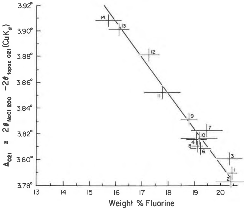
FIG. 4. \Delta_{021} \equiv 2\theta_{NaCl\ 200} - 2\theta_{topaz\ 021} as a function of fluorine content. Data from Table 1. Maximum error in measurement of \Delta_{021} is 0.005°. The equation of the regression line is in Table 2.
