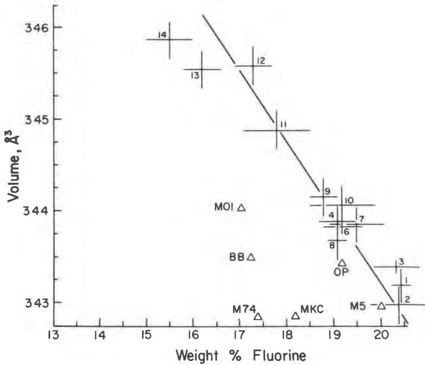
FIG. 3. (a) Variation of the b cell parameter and (b) unit-cell volume of topaz with fluorine content. Data from this paper (Table 1) and Rosenberg (1967) are represented by crosses whose sizes are indicative of the estimated standard errors of the measurements. The triangles represent data from Chaudhry and Howie (1970). Equations for the regression lines are listed in Table 2.
