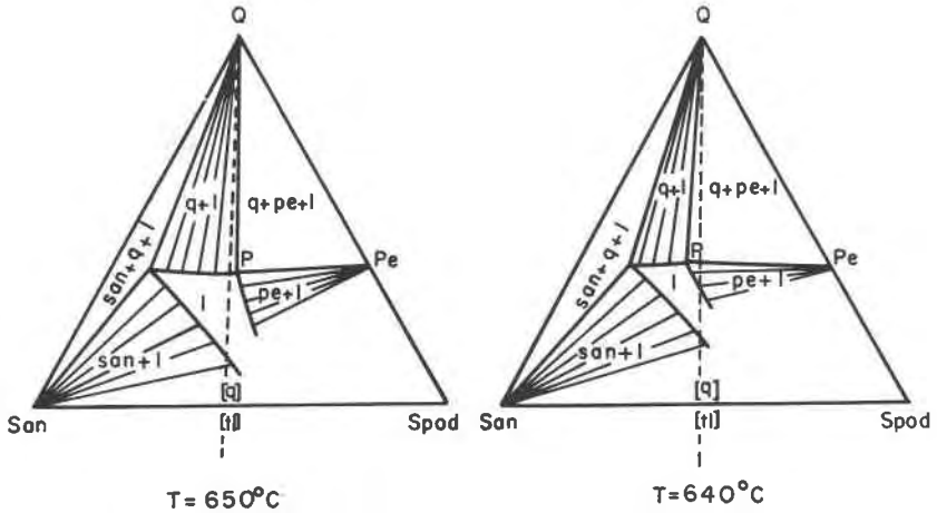
FIG. 6. Hypothetical phase relations in part of the system \text{KAlSiO}_4\text{-LiAlSiO}_4\text{-SiO}_2 at 2 kb. These isothermal diagrams are based on the interpretation of point P in the T\text{-}X section (Fig. 5). P represents the crossing of the element \text{LiQ} (quartz+petalite) over the \text{TL-Q} join. This implies the existence of a eutectic assemblage sanidine+petalite+quartz+liquid in the \text{San-Q-Pe} triangle, and on the \text{San} side of the \text{TL-Q} join. At 2 kb, the eutectic temperature is 600 \pm 10^\circ\text{C} . All tie lines and liquid compositions are schematic.
