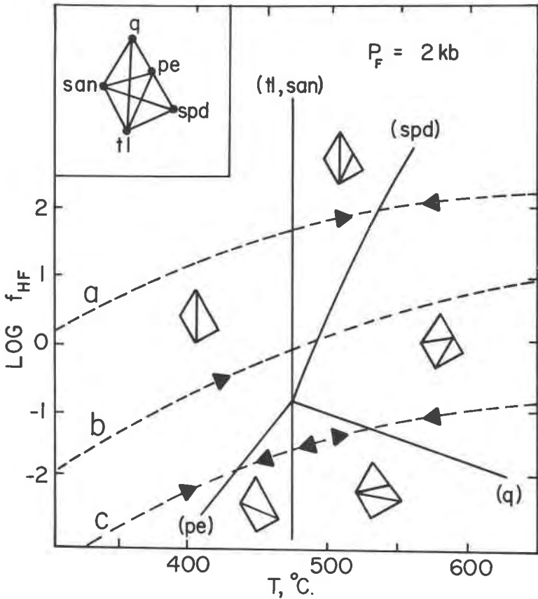
FIG. 7. \log f_{HF} - T showing sequence of univariant curves around the invariant point trillithionite (tl)+sanidine (san)+quartz (q)+petalite (pe)+spodumene (spd)+gas (g) at a total pressure of 2 kb. The approximate positions of the univariant curves have been established partly by the temperature of the reaction spodumene+quartz=petalite (480°C) and partly using the fluorine buffer technique to locate other curves. All boundaries have been reversed; arrows show direction from which equilibrium was approached. Dashed curves are the fluorine buffer assemblages: (a) NNO,OH(CFG,COHF), (b) NNO,OH(AFSQ,OHF), (c) MIC,COH(QFIC,COHF). For explanation of the notation of fluorine buffers, see Munoz and Eugster (1969).
