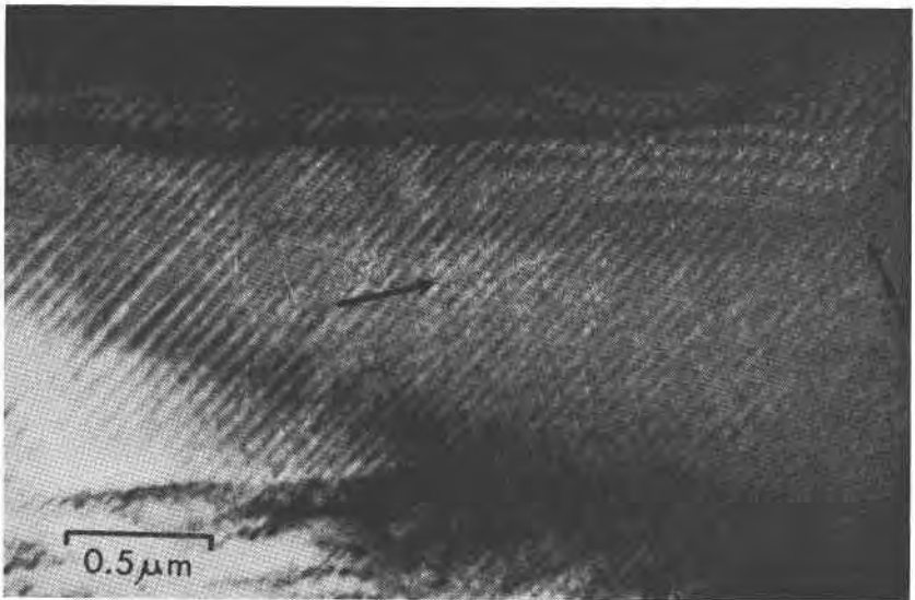
FIG. 3. Dark field micrograph of unetched solar flare particle tracks in a large (630 \mu\text{m} diameter) pyroxene fragment from the lunar soil which was sputter-etched after incorporation into a composite mount of epoxy resin and aluminum oxide powder. The exsolution lamellae in the pyroxene are seen as alternating black and white stripes. Two of the tracks are indicated by arrows.
