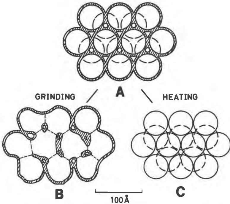
FIG. 7. Micromorphological model of allophane microaggregate. A: untreated, B: ground, c: heated. The oblique lines represent the water layer.
