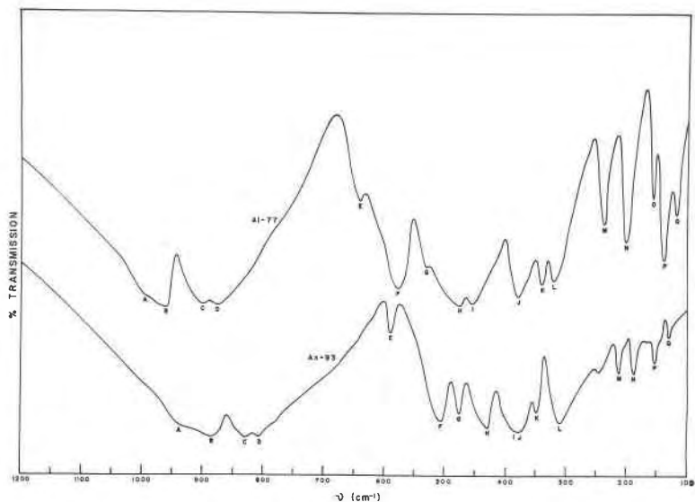
FIG. 1. Typical infrared spectra for an almandine (Al-77) and an andradite (An-93). The letter code on the bands refers to Table 2.
