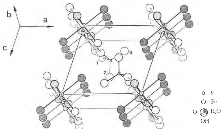
FIG. 1. Clinographic view of the structure of butlerite.
