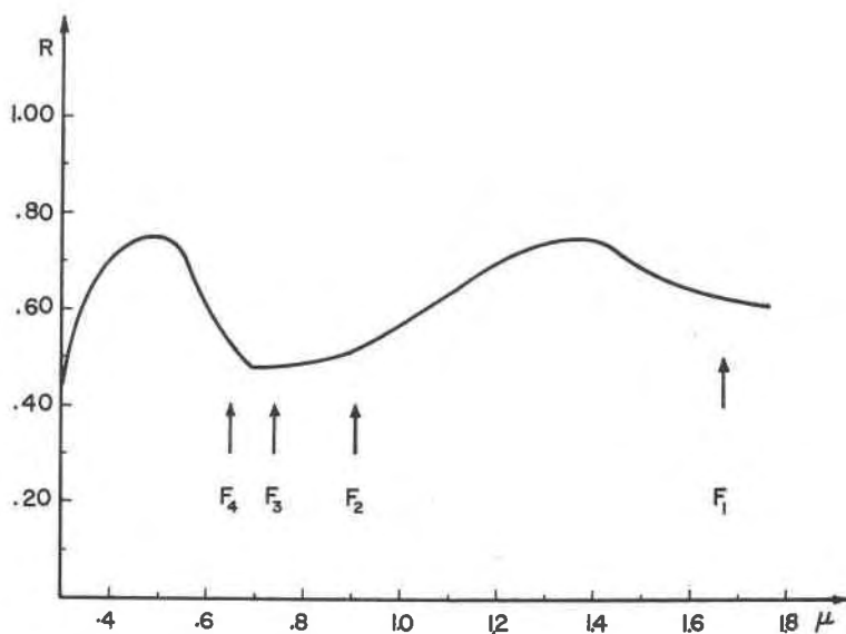
FIG. 2. Optical reflection spectrum of turquoise showing the reflectivity R as a function of the wavelength in microns.
