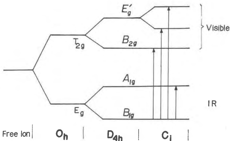
FIG. 4. Energy level splitting of the \text{Cu}^{2+} 3d^9, {}^2D electron configuration in an octahedral ( O_h ), tetragonal ( D_{4h} ), and lower symmetry ( C_i ) crystal field. Observed transitions are shown.
