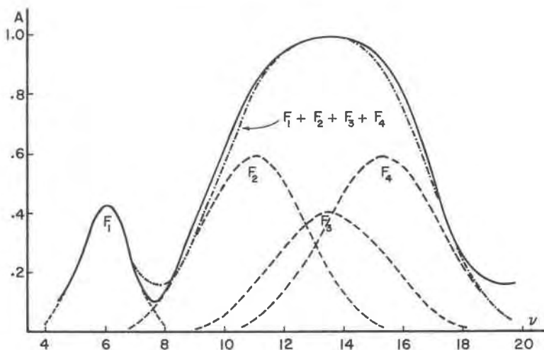
FIG. 3. The equivalent transmission spectrum of turquoise after converting from the experimental reflection spectrum. The abscissa is given in the units 10^3 \text{ cm}^{-1} .
