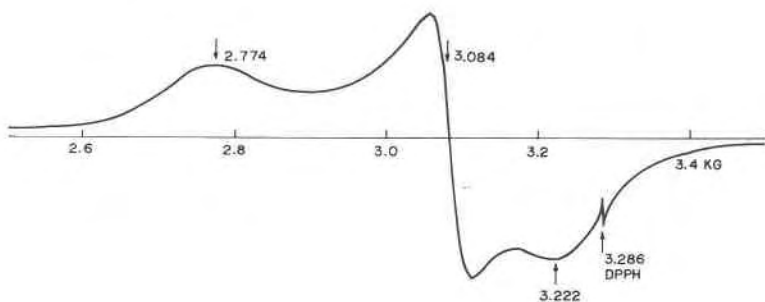
FIG. 1. Electron spin resonance spectrum of turquoise showing the location in kilogauss of the principal g -values g_1 , g_2 , g_3 , and that of the free radical marker DPPH.
