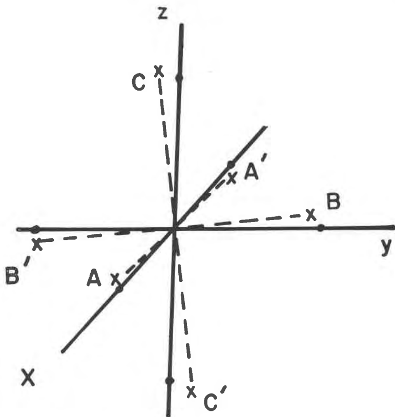
FIG. 5. Six atoms arranged in a slightly distorted octahedron with inversion symmetry.
