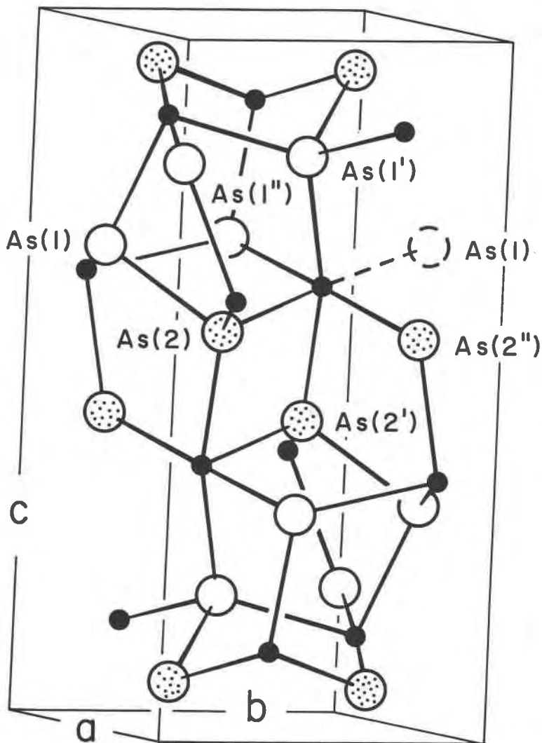
Fig. 1. The unit cell of paramammsbergite: As(1)—large circles; As(2)—large, stippled circles; Ni—small, full circles.
