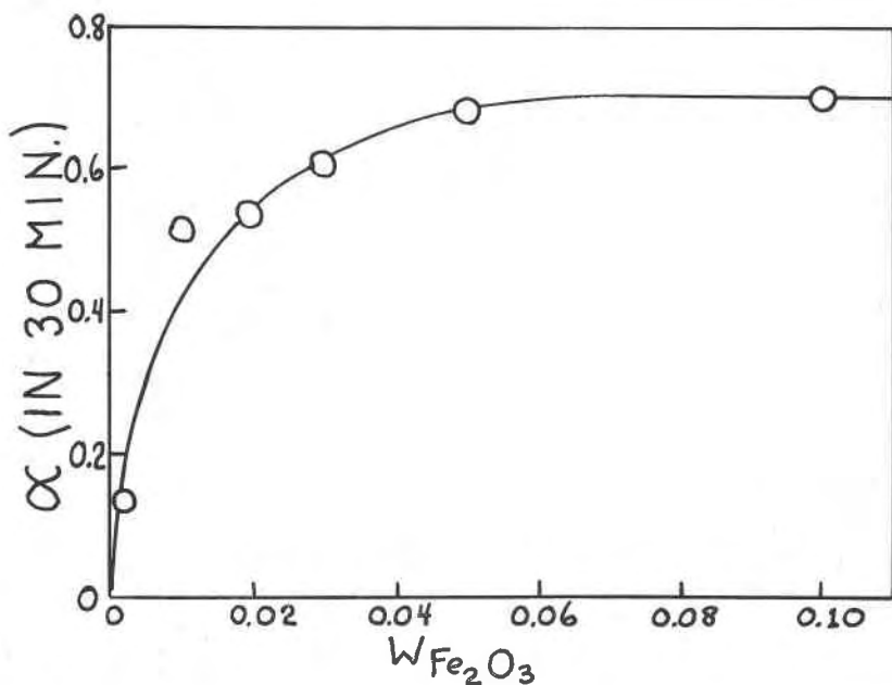
FIG. 8. Effect of high W_{\text{Fe}_2\text{O}_3} on the anatase/rutile transformation at 854^\circ\text{C} and 1 \text{ atm } \text{CO}_2/\text{H}_2 = 2.49 .
