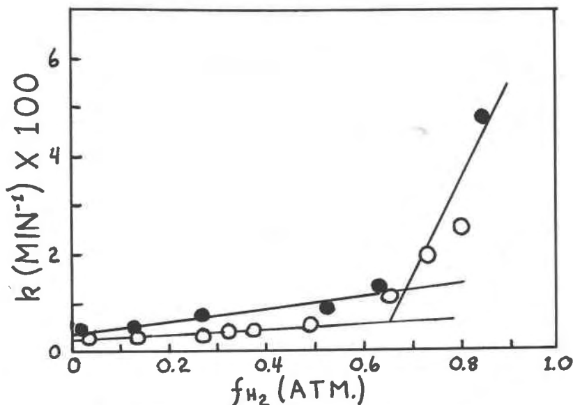
FIG. 7. Effect of hydrogen fugacity in CO_2/H_2 atmospheres on the anatase/rutile transformation at 1000^\circ C and 1 atm. Solid circles represent anatase plus 0.0294% hematite; open circles "pure" anatase.
