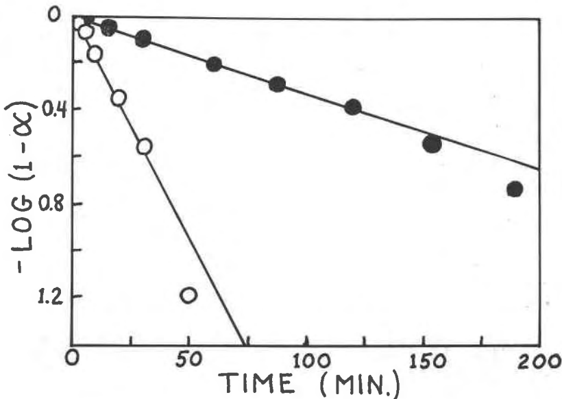
FIG. 2. Random nucleation equation plot, anatase/rutile transformation in the presence of 0.087% hematite at 1 atm. Open circles represent 1000°C and \text{CO}_2/\text{H}_2 = 27.4 ; solid circles 945°C and \text{CO}_2/\text{H}_2 = 2.75 .
