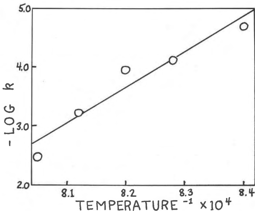
FIG. 4. Arrhenius plot, anatase/rutile transformation in the presence of 0.100% hematite. Pressure = 1 atm.; \text{CO}_2/\text{H}_2 = 2.49 . Rate constant k is from the phase boundary equation. The units of k are \text{min}^{-1} , and of temperature are ^\circ\text{K} .
