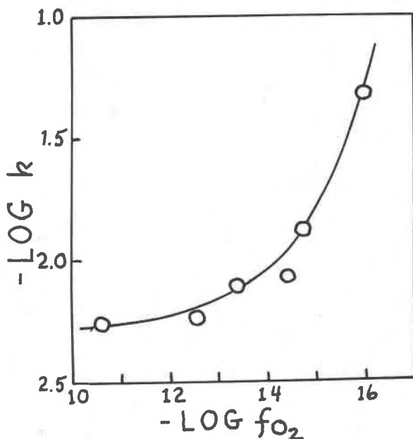
Fig. 6. Effect of reducing atmosphere, as expressed by oxygen fugacity, on the anatase/rutile transformation in the presence of 0.0294% hematite at 1000°C and 1 atm. Rate constant k is from the phase boundary equation; its units are \text{min.}^{-1}
