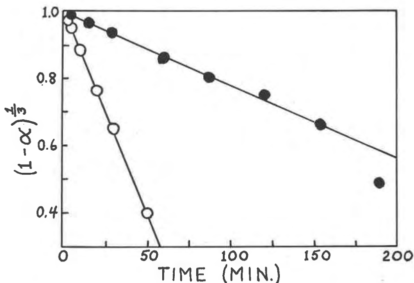
FIG. 3. Phase boundary equation plot, anatase/rutile transformation in the presence of 0.087% hematite at 1 atm. Open circles represent 1000°C and \text{CO}_2/\text{H}_2 = 27.4 ; solid circles 945°C and \text{CO}_2/\text{H}_2 = 2.75 .
