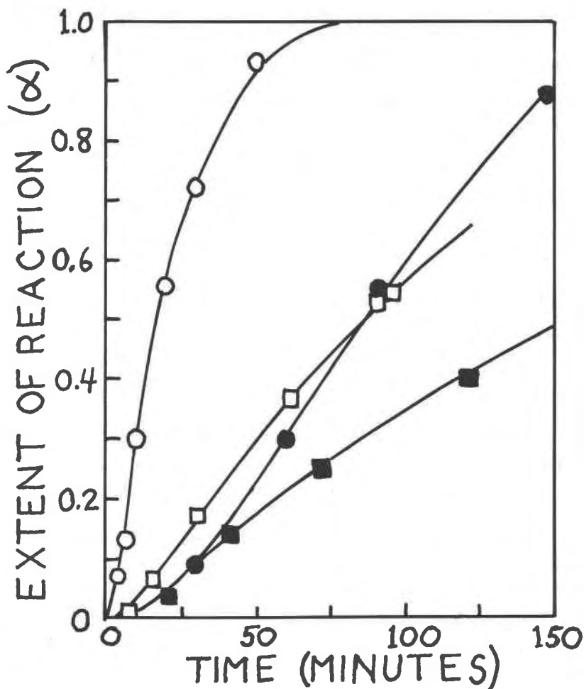
FIG. 1. Extent of reaction ( \alpha ) of the anatase/rutile transformation at 1000°C and 1 atm. Solid squares represent "pure" anatase in air; solid circles anatase plus 0.087% hematite in air; open squares "pure" anatase in \text{CO}_2/\text{H}_2 = 27.4 ; open circles anatase plus 0.087% hematite in \text{CO}_2/\text{H}_2 = 27.4 .
