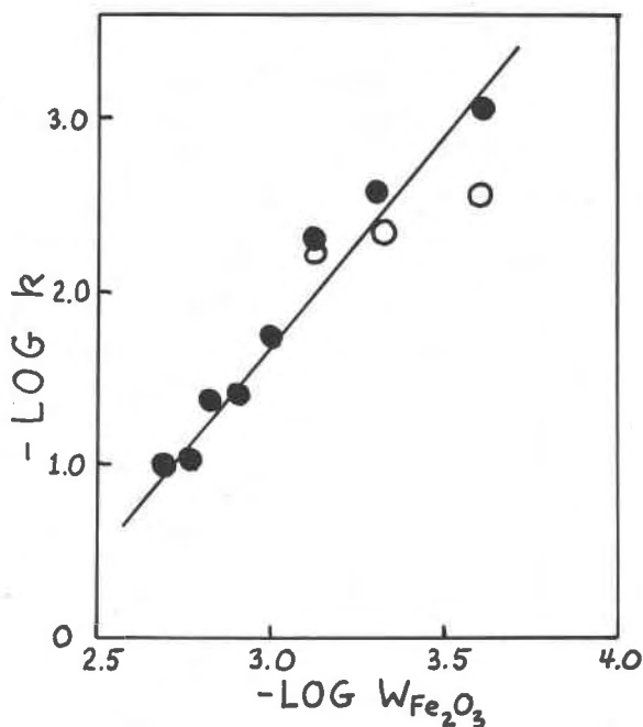
FIG. 5. Effect of the weight fraction of hematite ( W_{\text{Fe}_2\text{O}_3} ) on the anatase/rutile transformation at 946^\circ\text{C} and 1 atm. \text{CO}_2/\text{H}_2 = 2.49 . Rate constant k is from the phase boundary equation; its units are \text{min.}^{-1} . Points represented by black circles have been corrected for the reaction in pure anatase; those represented by open circles have not.
