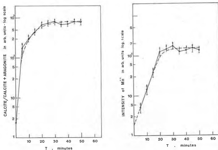
Fig. 5. (a). The concentration of calcite, as determined by X-rays in aragonite samples, as a function of heating time at 430^{\circ}C . (b). The intensity of the Mn^{2+} spectrum as a function of heating time. Notice that both curves show saturation behavior at approximately the same time. The dotted curves are an average through the experimental points.
