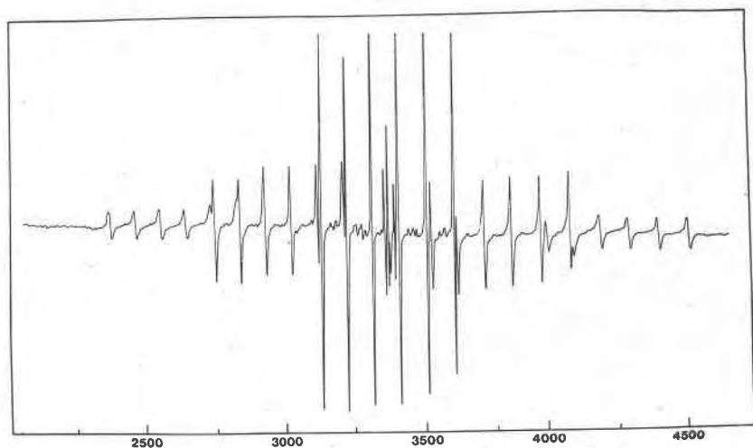
Fig. 4. The ESR spectrum of Mn^{2+} in aragonite with the magnetic field along the crystallographic b axis. Note that all the inequivalent sites coincide and only 30 lines are to be seen.
