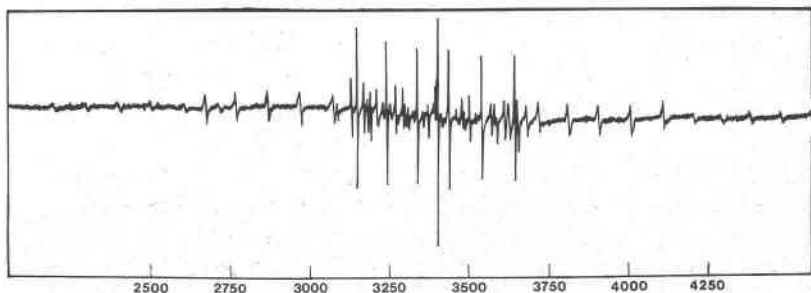
FIG. 3. The ESR spectrum of Mn^{2+} in single crystal aragonite (Aragon, Spain). The crystal was heated to 300^\circ C for a few hours. The magnetic field is along the magnetic z axis. Compare with Figure 1. The spectrum consists of 60 lines; 30 lines spread over approximately 2,000 gauss and 30 lines fall approximately within the six intense hyperfine lines within 600 gauss.
