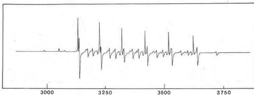
FIG. 2. The ESR spectrum of Mn^{2+} spectrum in powered calcite samples (Iceland spar). The six intense hyperfine lines correspond to the six strong hyperfine lines in Figure 1. It is to be noted that they are double. The doubling arises because of the magnetic inequivalences of the two ions. The weaker outer lines arise from the remnants of the fine structure lines shown in Figure 1. The main six hyperfine lines are shifted in Figure 2 from those of Figure 1, because of the different setting of the operating frequency of the spectrometer.
