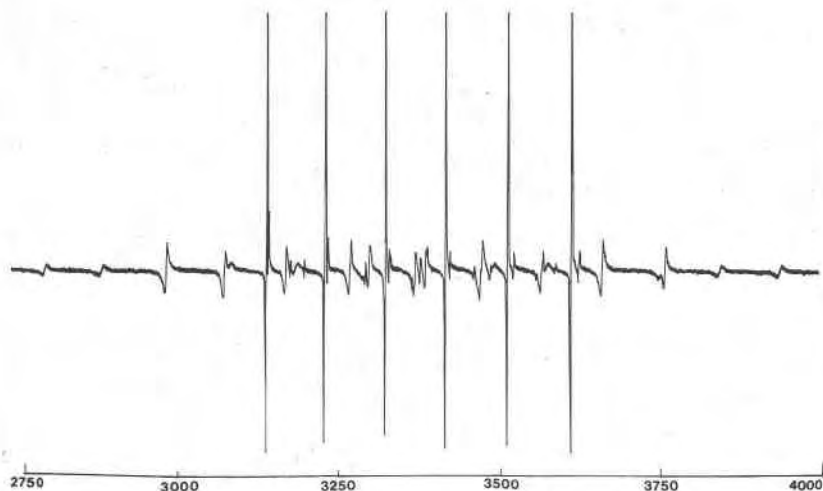
FIG. 1. The ESR spectrum of Mn^{2+} in single crystals of calcite (Iceland spar). The spectrum is taken at 3 cm wavelength and with the magnetic field parallel to magnetic z axis. The lines in Iceland spar are particularly sharp.
