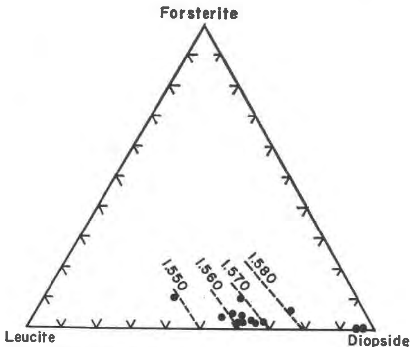
FIG. 5. Isofrac lines in the system forsterite-diopside-leucite.
