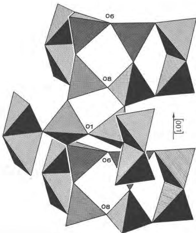
FIG. 3. A polyhedral representation of the [\text{Si}_6\text{O}_{15}]_n double-chain of epididymite (stippled) and associated \text{Be}_2\text{O}_6 groups (ruled).
