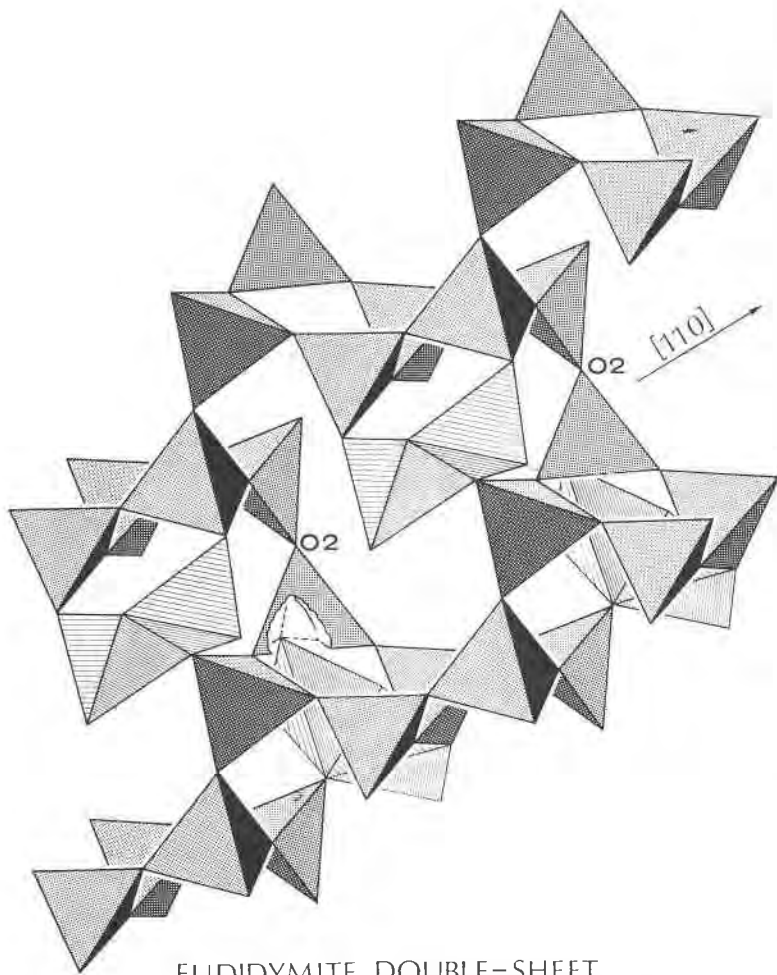
FIG. 2. A perspective polyhedral drawing of the eudidymite double-sheet which parallels (001). Stippled tetrahedra represent \text{SiO}_4 groups and ruled tetrahedra depict \text{BeO}_4 groups. The sharing of the "double chains" through O(2), in forming double sheets, can be clearly seen.
