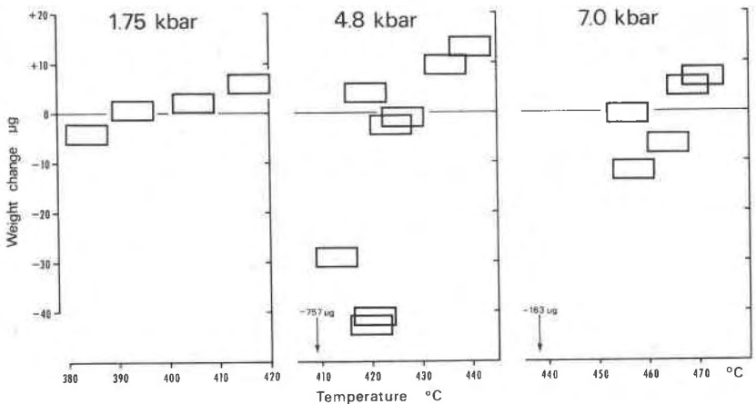
FIG. 2. Observed weight changes of single crystals of corundum at pressures not shown in Figure 1. The interpretation of these data is represented by horizontal bars along the equilibrium curve No. 1 in Figure 3. To improve clarity the error field for each experiment is reduced to about half of the actual temperature uncertainty of \pm 5^\circ .
