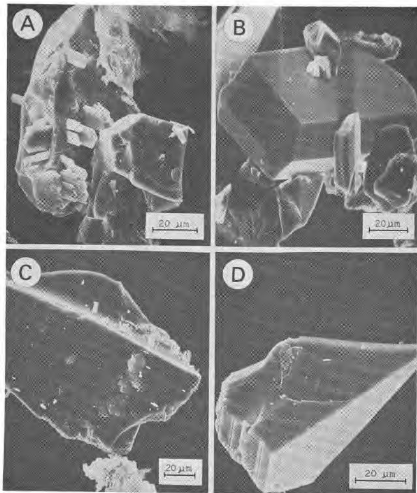
FIG. 4. Scanning electron photomicrographs. (A) Corundum grain after run of 50 days at 2.4 kbar and 380° C, 25° below the equilibrium temperature. Diaspore is growing epitaxially in two directions in the 0001 plane of corundum (the third direction is not visible in this picture). Orientations: c of corundum and a of diaspore vertical on picture, c of diaspore parallels elongation. (b) Euhedral diaspore crystal, nucleated and grown in 30 days at 2.4 kbar and 367° C, 38° below equilibrium temperature. Orientation of crystal: c horizontal, b approximately vertical and perpendicular to largest surface. (C) Diaspore growing on corundum grain. The spines are ca. 8 μm long and grew at 2.4 kbar and 401° C in 29 days, 4° below equilibrium temperature. (D) Corundum grain showing growth pattern which developed in 30 days at 2.4 kbar and 407° C, 2° above equilibrium temperature.
