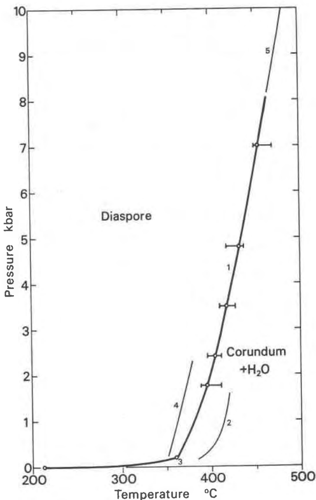
FIG. 3. Equilibrium curves for the reaction \text{diaspore} \rightleftharpoons \text{corundum} + \text{water} . No. 1: This report, between 390° and 470° C based on experimental data, from 220° to 390° C based on calculations. Horizontal bars indicate range of possible equilibrium temperature at each experimental pressure. No. 2: Reported by Ervin and Osborn (1951). No. 3: Equilibrium point by Fyfe and Hollander (1964). No. 4: Hydrothermal results of Kennedy (1959). No. 5: Piston-anvil results of Kennedy (1959).
