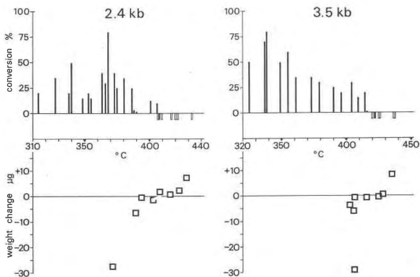
FIG. 1. Experimental results at 2.4 and 3.5 kbar. Top : Solid bars pointing upward represent percentage of corundum powder which converted to diaspore crystallites. Open bars pointing downward indicate temperature at which no diaspore growth can be detected. Solid bars pointing downward show runs where scanning electron photomicrographs were made and growth of corundum could be detected. Bottom : Squares indicate weight change of single corundum crystals during 30 days runs. For improved clarity the symbols to indicate weight change are drawn smaller than the actual tolerance range would require. Tolerances are \pm 3 \mu\text{g} for the weight change. Thus the boxes should be about twice the drawn size. Considering both investigations the equilibrium temperature at 2.4 kbar is 405^\circ \text{C} \pm 7^\circ and at 3.5 kbar 418^\circ \text{C} \pm 7^\circ .
