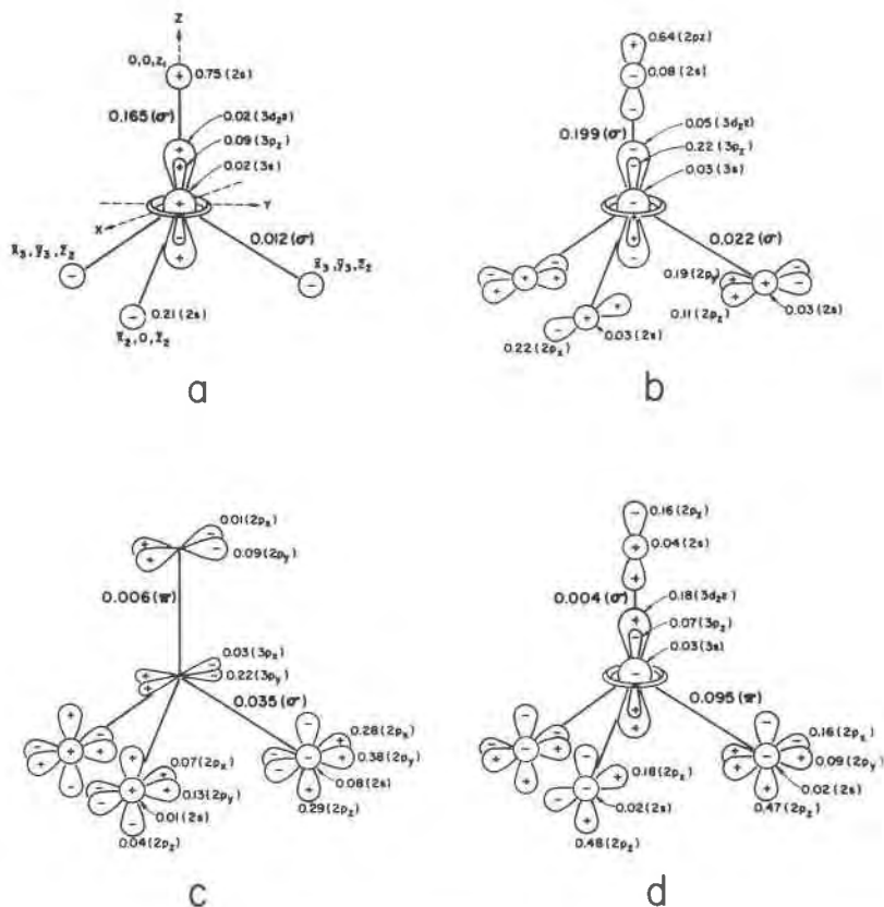
FIG. 8. Schematic representation of the STO-AO components of the molecular orbitals for a orthosilicic acid molecule of C_{3v} symmetry with \alpha = 117^\circ and all Si-O = 1.63\text{\AA} . Hydrogen orbitals are omitted. (a) represents the AO components of the 2a_1 MO, (b) of the 4a_1 MO, (c) of the 2e MO with 3d components suppressed, and (d) of the 5a_1 MO. The bold-face numbers indicate the partial overlap population that these MOs contribute to the total n(Si-O) .
