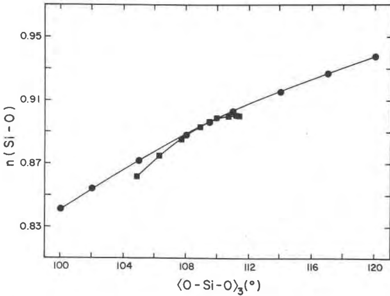
FIG. 7. Variation of n[\text{Si-O (apical, circles)}] and n[\text{Si-O (basal, squares)}] as a function of \langle \text{O-Si-O} \rangle_3 for the \text{H}_4\text{SiO}_4 molecule ( C_{3v} symmetry, all Si-O = 1.63Å, and with Si( spd ) basis set).
