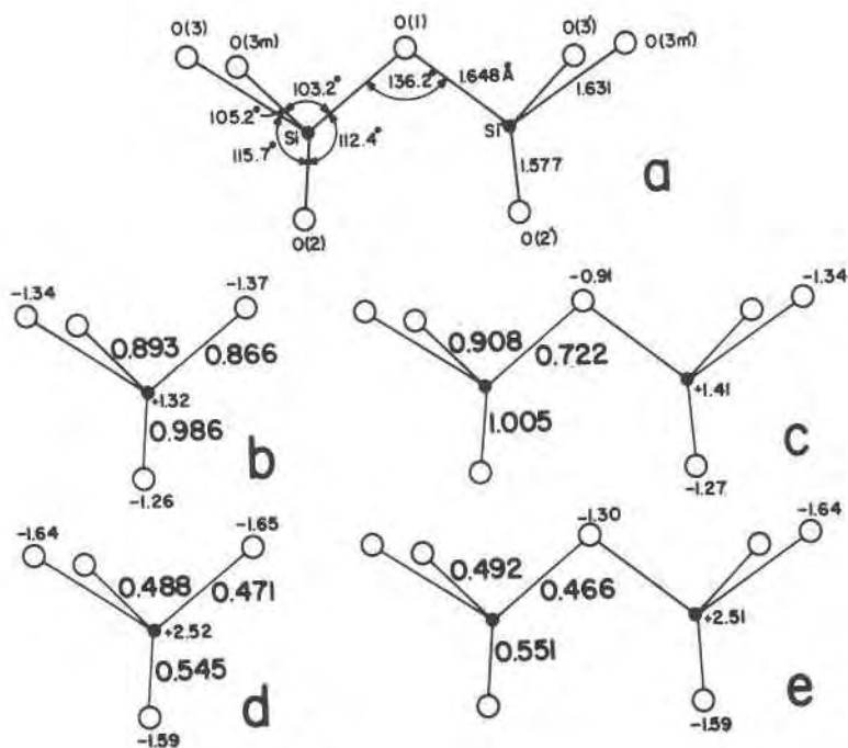
FIG. 9. Results of EHMO calculations for the (\text{Si}_2\text{O}_7)^{6-} ion in sodamelilite. (a) Dimension of the pyrosilicate ion. (b) n(\text{Si-O}) and Q(r) for the "hypothetically isolated" (\text{SiO}_4)^{4-} group, and (c) for the actual (\text{Si}_2\text{O}_7)^{6-} group with \text{Si}(sp^3d) basis set. (d) and (e) are similar results for \text{Si}(sp) basis set calculations.
