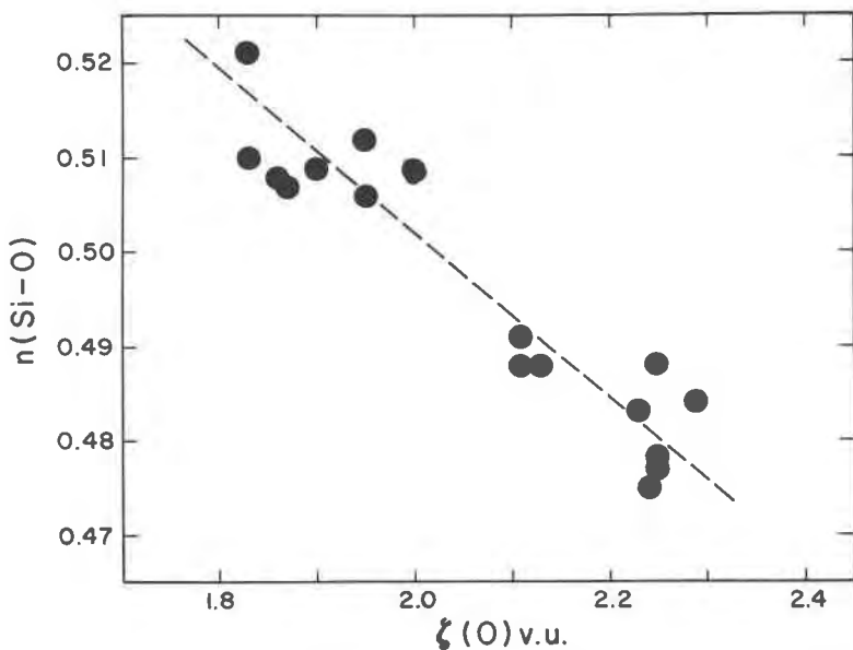
FIG. 6. \zeta(\text{O}) vs. n(\text{Si}-\text{O}) for tetrahedral bond lengths in tourmaline and margarosanite. n(\text{Si}-\text{O}) values, calculated with the \text{Si}(\text{sp}) basis set with Si-O clamped at 1.63\text{\AA} , are from Gibbs et al. (1972).
