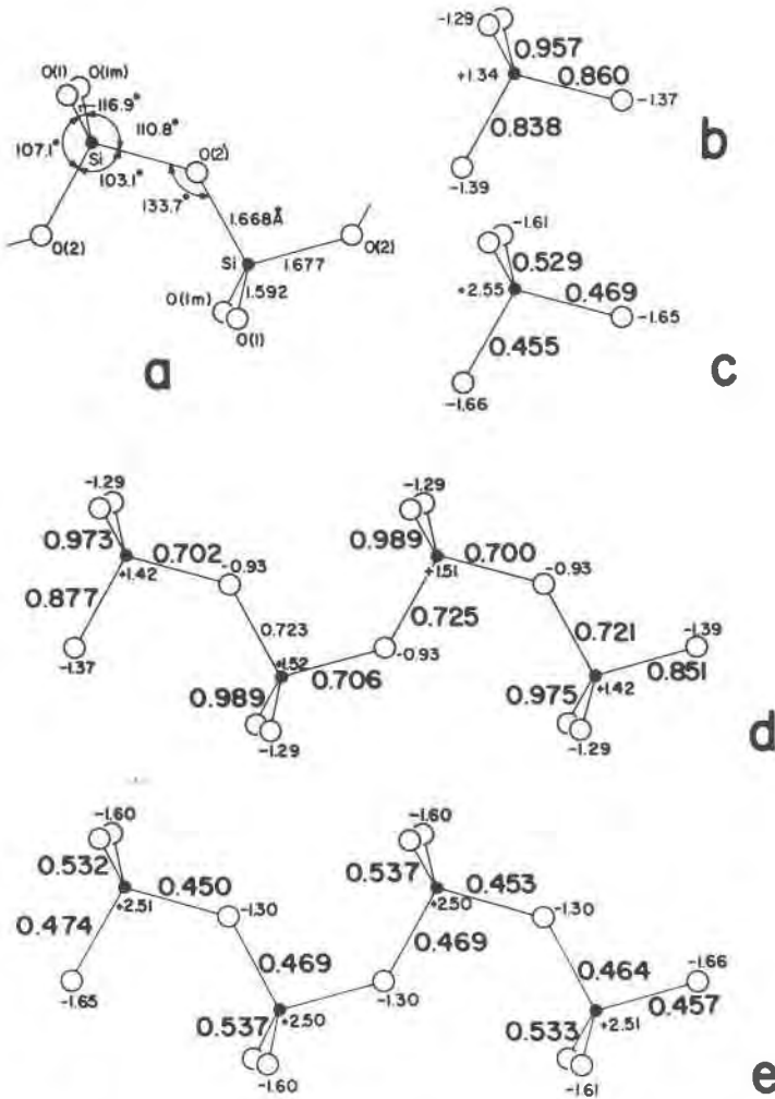
FIG. 10. Results of EHMO calculations for the (\text{SiO}_3)_\infty single chain in \text{Na}_2\text{SiO}_3 . (a) Dimensions of the chain. (b) n(\text{Si}-\text{O}) and Q(r) for the hypothetically isolated (\text{SiO}_4)^{4-} group calculated with \text{Si}(spd) and (c) \text{Si}(sp) basis sets. (d) and (e) are similar calculations for a four-membered single chain.
