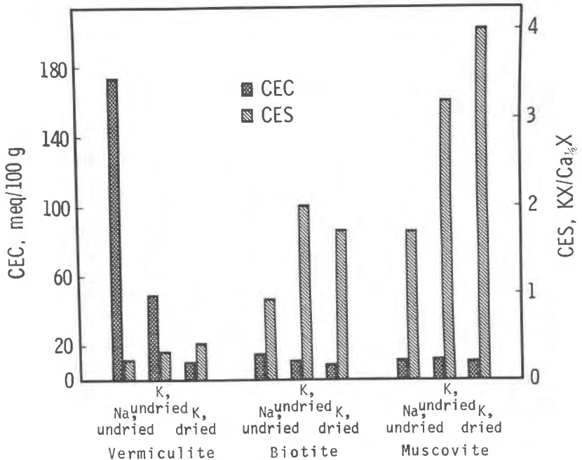
Fig. 1. CEC and \text{K}/\text{Ca} CES for sodium saturated (undried), potassium saturated (undried), and potassium saturated then dried vermiculite, biotite, and muscovite.
