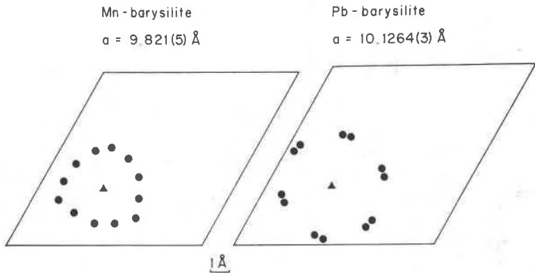
FIG. 2. Schematic representation of channel cross-sections comparing Mn-barysilite (Lajzerowicz, 1966) and Pb-barysilite (Petter et al. , 1971) in a (001) projection. Only the centers of the oxygen atoms forming one channel are shown. The position of the X atoms is on the 3 axis.
