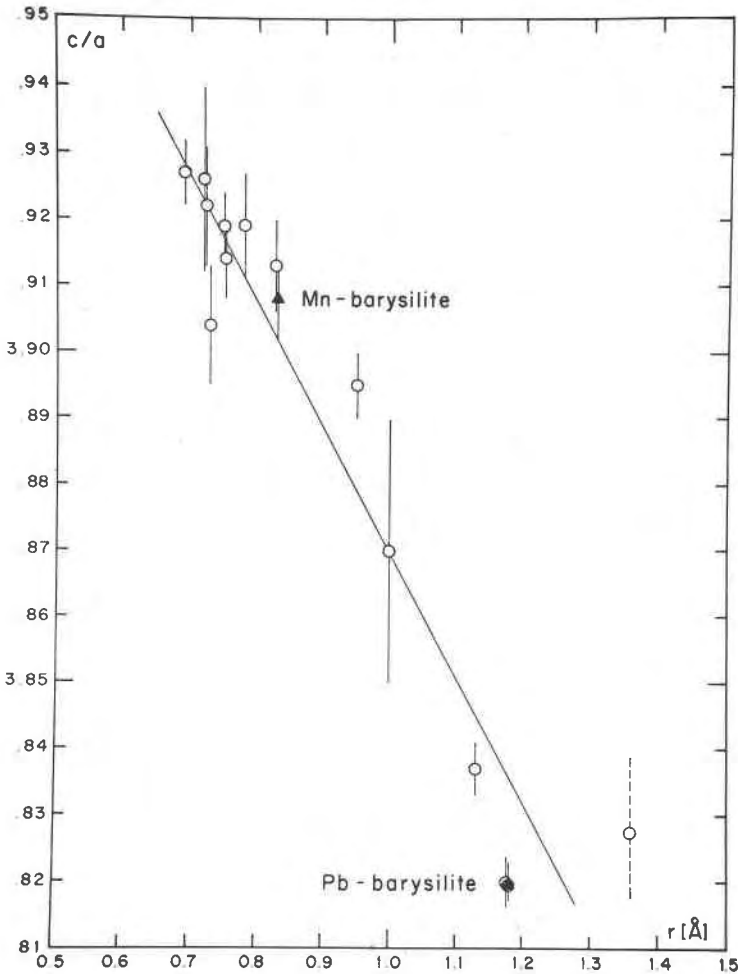
FIG. 1. Plot of the axial ratio c/a versus the divalent ionic radius r (Shannon and Prewitt, 1969) for six-coordinated metal cations at the X site. The correlation coefficient \hat{R} = -0.96 . Triangles indicate compounds whose structures have been determined, circles other data from Table 1. The vertical bars are estimated standard errors, except for the lower right data point whose errors were not reported.
