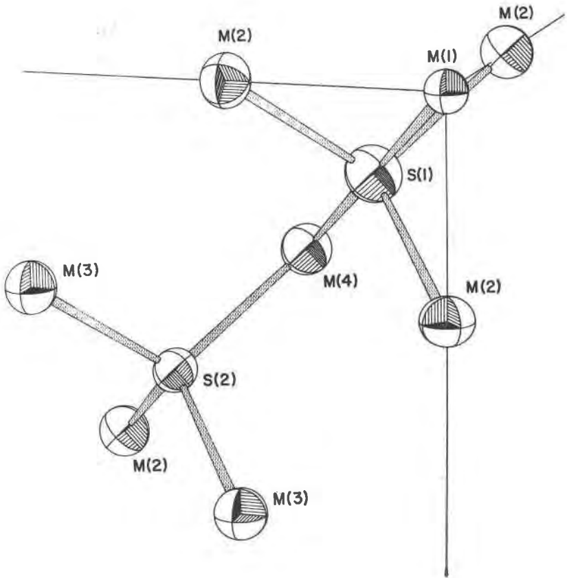
FIG. 3. A partial structural model of talnakhite showing the atomic thermal ellipsoids of model A plotted at the 90 percent probability level.
