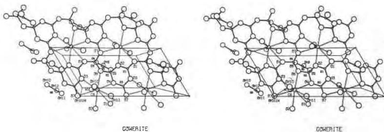
FIG. 1. Stereoscopic-pair view along b of one polyoxoanion sheet, [B_6O_6(OH)]^{2-} , in gowerite. The outline of one unit cell is shown with a horizontal. Ca coordination is indicated by double lines. W1 designates a water molecule.
