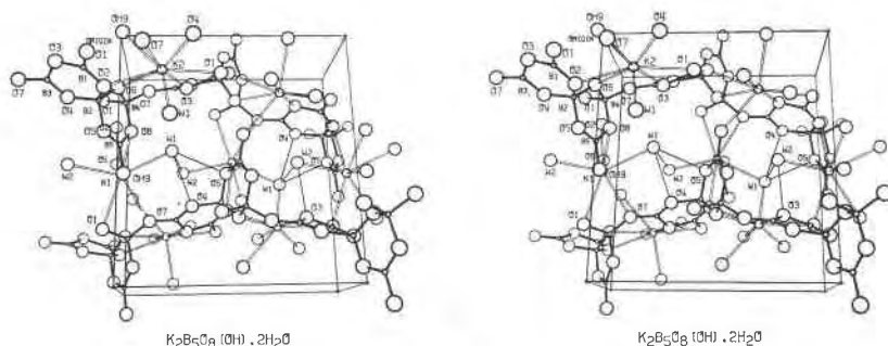
FIG. 3. Stereoscopic-pair view along b of a part of the synthetic K_2B_5O_8(OH) \cdot 2H_2O structure to illustrate the intersheet linkages; data from Marezio (1969). The outline of one unit cell is shown with c horizontal; a rotation of 20° around c was made for clarity. W designates the water molecules; hydrogen bonds are drawn by light, thin lines.
