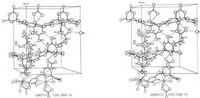
FIG. 2. Stereoscopic-pair view of a part of the gowerite structure along c^* to show the stacking of sheets and the intersheet linkages. The outline of one unit cell is shown with a horizontal. W designates the water molecules; hydrogen bonds are drawn with light, thin lines.
