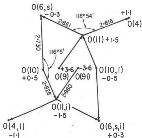
FIG. 6. Proposed hydrogen bonding scheme with distances and angles in the leucophosphite structure. The tails of the arrows are located at the donors and the heads at the acceptors. The scheme is located at the inversion center of the tetramer in Fig. 2.
