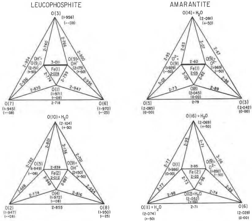
FIG. 3. Interatomic distances and anionic deviations from electrostatic neutrality in the leucophosphite octahedra and the amarantite octahedra. The tabulations are presented as Schlegel diagrams, which can be directly compared by super-position. Shared edges are drawn bold; Me-O distances and \Delta\Sigma are listed parenthetically. The average Me-O distance is underlined. Estimated standard errors are Me-O \pm 0.005 and O-O' \pm 0.007 Å. The amarantite data are from Süsse (1968). i = inversion, s = screw operations applied to the atomic coordinates in Table 2.
