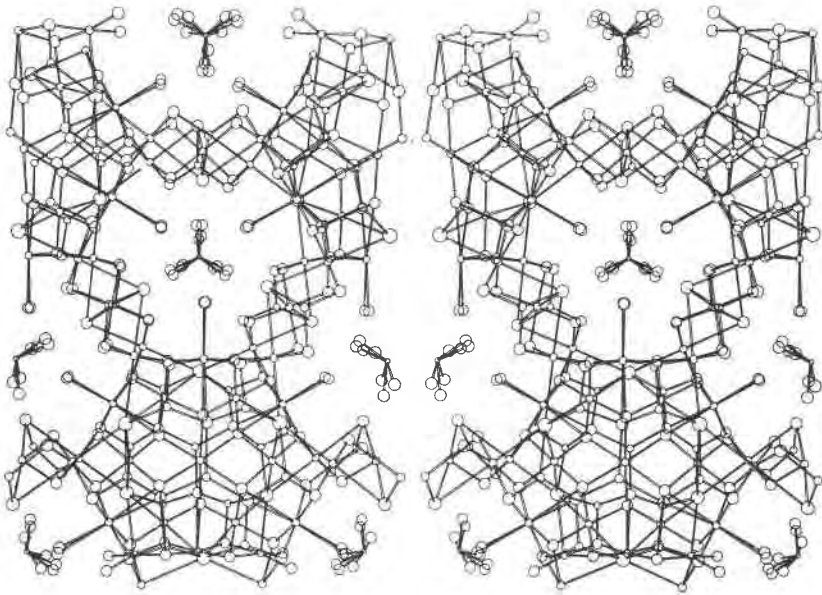
FIG. 3. Structure as in Fig. 1 viewed in stereo illustrating the blend of intricate detail and overall simplicity that is connellite. Shown are one complete narrow channel (1, 1, z ) and one complete large channel ( 1/3 , 2/3 , z ).
