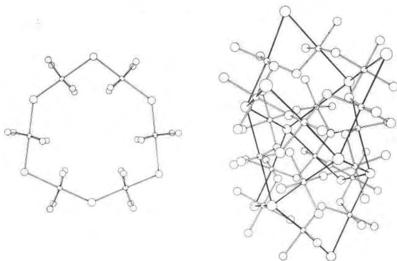
FIG. 4. Structural elements in connellite. A. Ditrigronal ring composed of Cu(2) and Cu(2A) polyhedra. The more obtuse angles of the ring are at Cl and the less obtuse at O(7). View direction is parallel to c . B. Cylindrical diamond-shaped network in the structure of connellite composed of Cu(1) and Cu(1A) polyhedra. Cu-Cl bonds are stressed to accent the diamond shape formed by the long axes of the polyhedra. View direction is at 45^\circ to the c axis.
