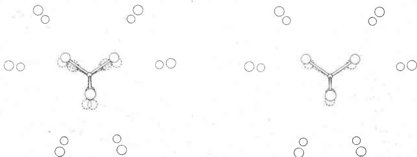
Fig. 5. The sulfate disorder in connellite. A. Three-fold disorder resulting from the occupation of a \bar{b} site by the less symmetrical (\text{SO}_4)^{2-} ion. One of the three orientations is indicated by full lines and the alternative orientations by dashed lines. B. Substitutional disorder resulting from the substitution of (\text{NO}_3)^- for (\text{SO}_4)^{2-} . One of the three sulfate orientations is shown by full lines and the superimposed nitrate by dashed lines.
