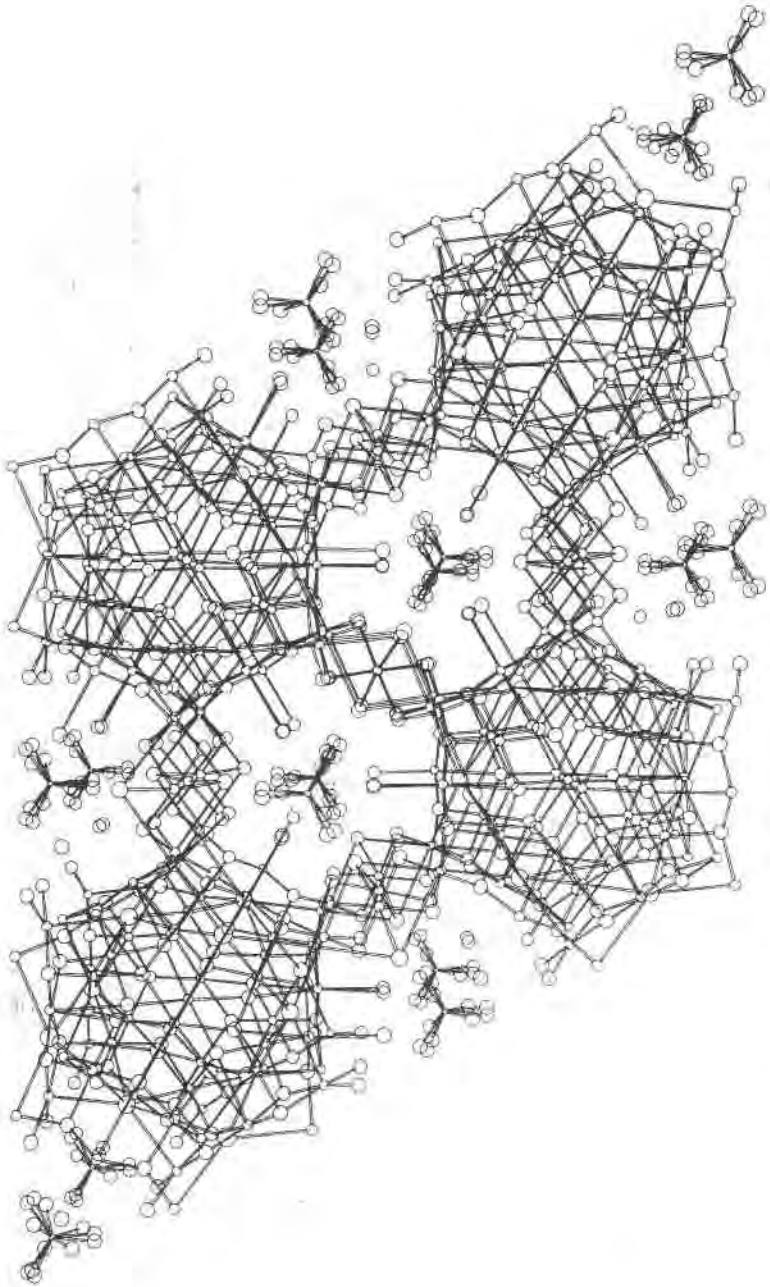
Fig. 2. Structure as in Fig. 1 viewed in perspective illustrating its intricacy when considered in detail.
