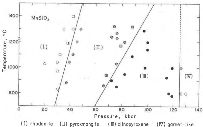
FIG. 1. Synthesis diagram for the high-pressure and high-temperature transformations of \text{MnSiO}_3 . Starting materials are \text{MnSiO}_3 I, rhodonite, except for reverse reaction runs indicated by squares.
