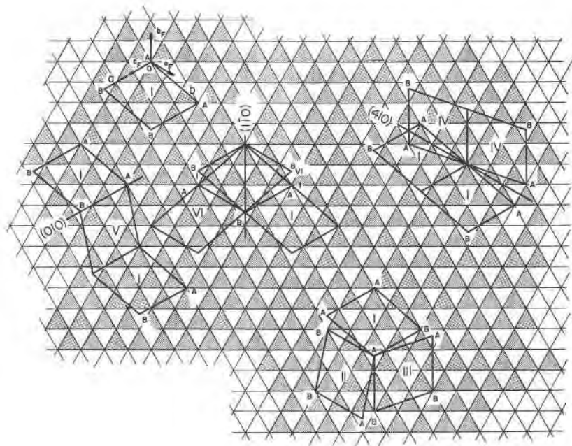
FIG. 4. Unit cell, edges of the F -centered cubic subcell and four observed twin laws of synthetic sinnerite on a background of the cubic substructure of sinnerite. Projection along the c -axis, perpendicular to the ABC layer stack of tetrahedra of the cubic sphalerite-like substructure with the tetrahedra of the A layer shaded. A and B indicate the position of the ends of the unit cell vectors with respect to the layers when the origin is situated in the A layer.
