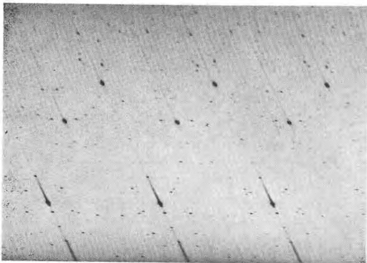
FIG. 2. Zero-level Weissenberg photograph of a sinnerite composite twin. Strong reflections belong to six closely overlapping pseudocubic subcells and weak reflections to six triclinic sinnerite lattices. The relationships may be traced with a help of Figure 3.
