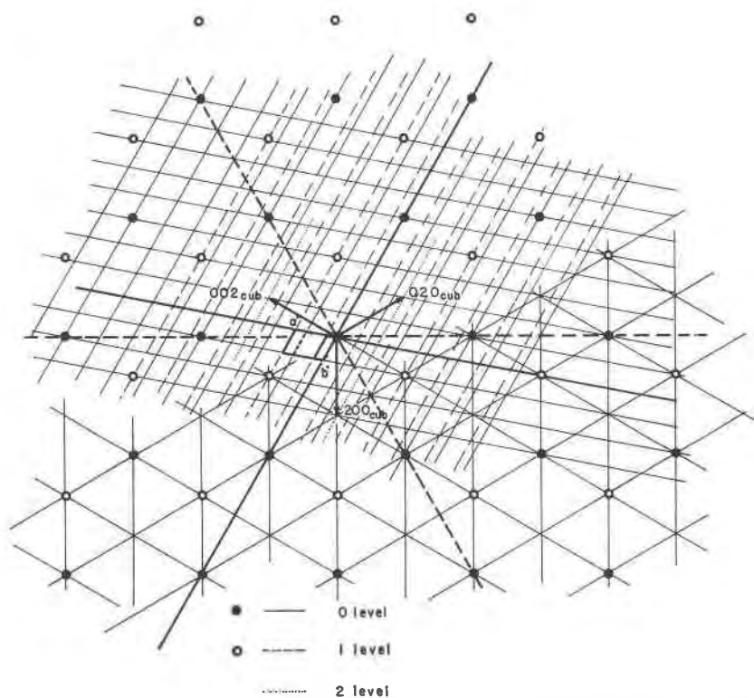
FIG. 3. Zero and first levels of the reciprocal lattice of sinnerite. Nodes of the cubic sublattice are denoted by circles. Reciprocal cell of sinnerite (in a projection on the a^* \cdot b^* plane) and edges of the cubic reciprocal subcell are given in heavy outlines at the origin.
