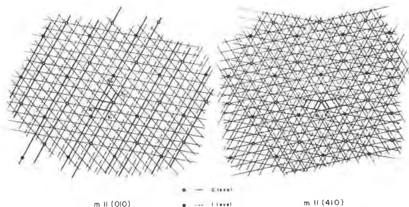
FIG. 5. Manifestation of the twinning on planes (010) and (410) in the reciprocal space. Zero and first levels of the reciprocal lattice of sinnerite are given. Subcell nodes denoted by circles, true-cell by the intersections of the reciprocal-lattice grid. Reciprocal unit cells of the two twin individuals (in projection on the a^* \cdot b^* plane) and overlapping rows of the reciprocal lattices of them are indicated by heavy solid lines for both levels.
