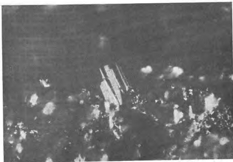
FIG. 1. Composite prism of synthetic sinnerite grown at 450°C with re-entrant angles. Length 0.1 mm.
