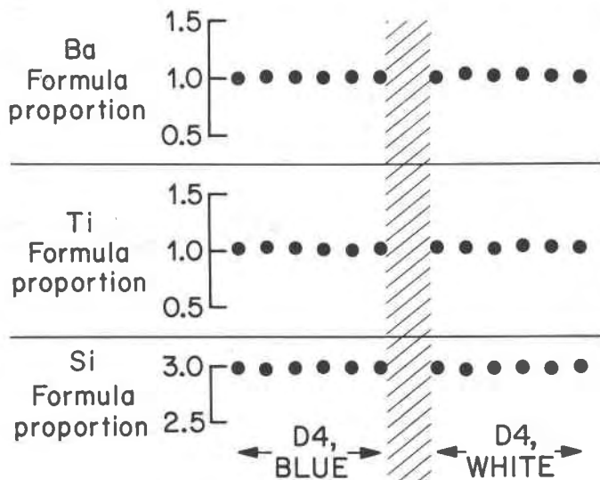
FIG. 1. Scatter diagram for the cation formula proportions of benitoite samples from San Benito County, California. Each point represents a complete microprobe analysis. Formula proportions are determined by normalizing the analyses to anhydrous oxygen = 9.
