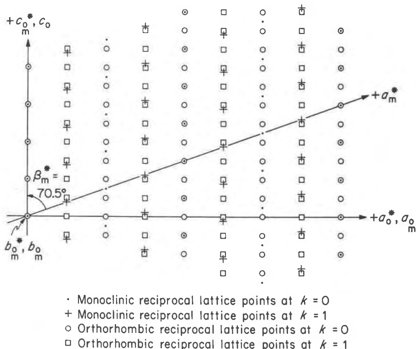
FIG. 4. Relationship between the orthorhombic (o) and monoclinic (m) reciprocal lattices of joaquinite. Reciprocal axes are shown by the symbol *.
