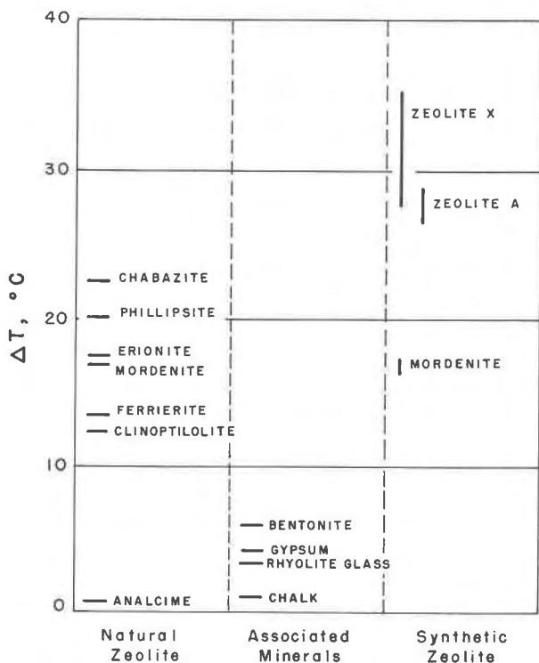
FIG. 2. Temperature data obtained by field kit measurements on natural zeolites, associated minerals, and synthetic zeolites, corrected for impurities.
