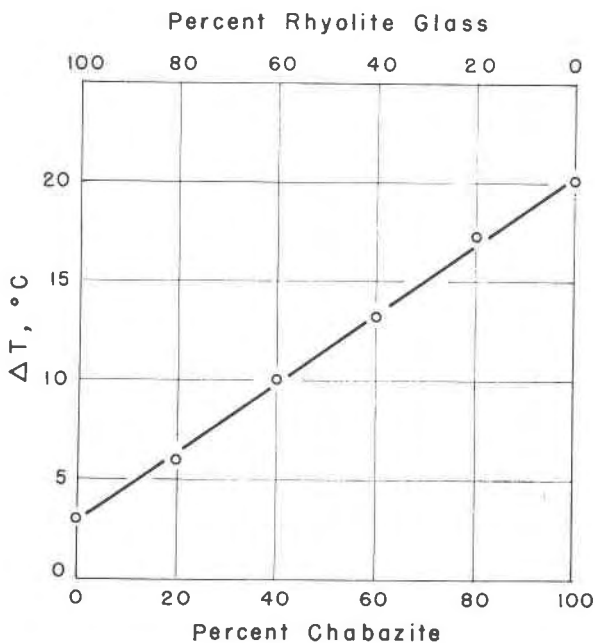
FIG. 3. Temperature data obtained on prepared mixtures of natural Na, K-chabazite and partially altered rhyolite glass.
