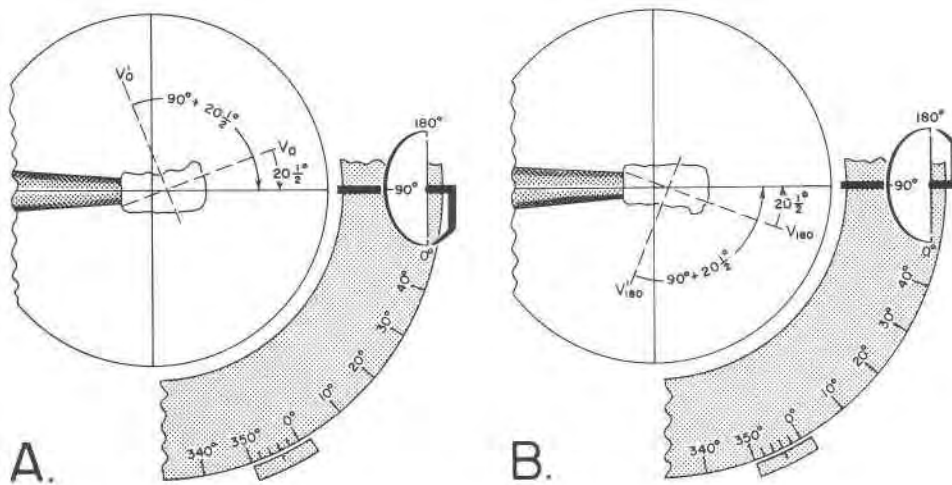
FIG. 1. (A) Sample field of view imposed on a schematic partial drawing of the microscope stage and spindle as seen after the spindle (set to read S = 0^\circ ) has been visually aligned with the E-W crosshair, the spindle tip pointing west. (The reversal of images by the microscope makes the tip appear to point east within the field of view). A low-power objective, if used, will permit more of the spindle to be seen within the field of view during the alignment. As shown, M_E equals 356^\circ for this example.
