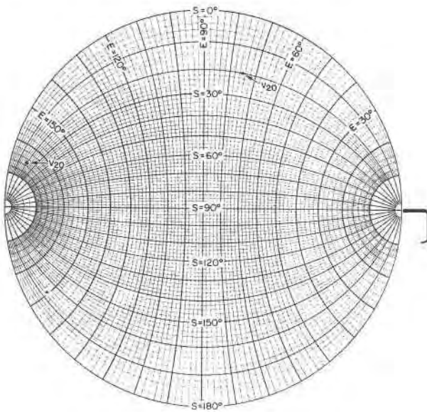
FIG. 3. Orientation of stereonet used for plotting a crystal's vibration directions if their S , E_s coordinates are known.
