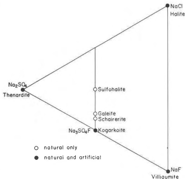
FIG. 8. Minerals in the system \text{Na}_2\text{SO}_4 - \text{NaF} - \text{NaCl} . Compositions plotted in terms of mole proportions.
