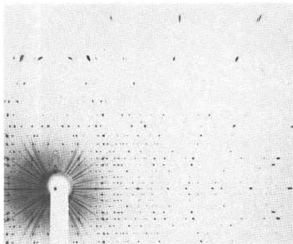
FIG. 1. The X-ray rotation pattern of a kogarkoite crystal grown from solution at 38°C. Cu radiation, Ni filter. Rotation axis [102] monoclinic, corresponding to c pseudohexagonal. c^* streaks visible adjacent to strong spots on 80\bar{8}l locus on which spots appear only on layer lines for which l \neq 3n in accordance with requirements of rhombohedral centering.
