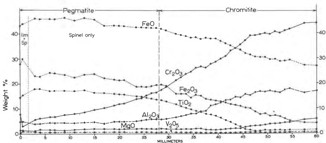
FIG. 12. Microprobe traverse from chromitite across the magnetic spinel layer of Figure 11. The long dashed vertical line is the pegmatite-chromitite contact. Each vertical line of points represents an analysis at a point along the traverse. Ilmenite coexists with spinel at points to left of the short-dashed vertical line.
