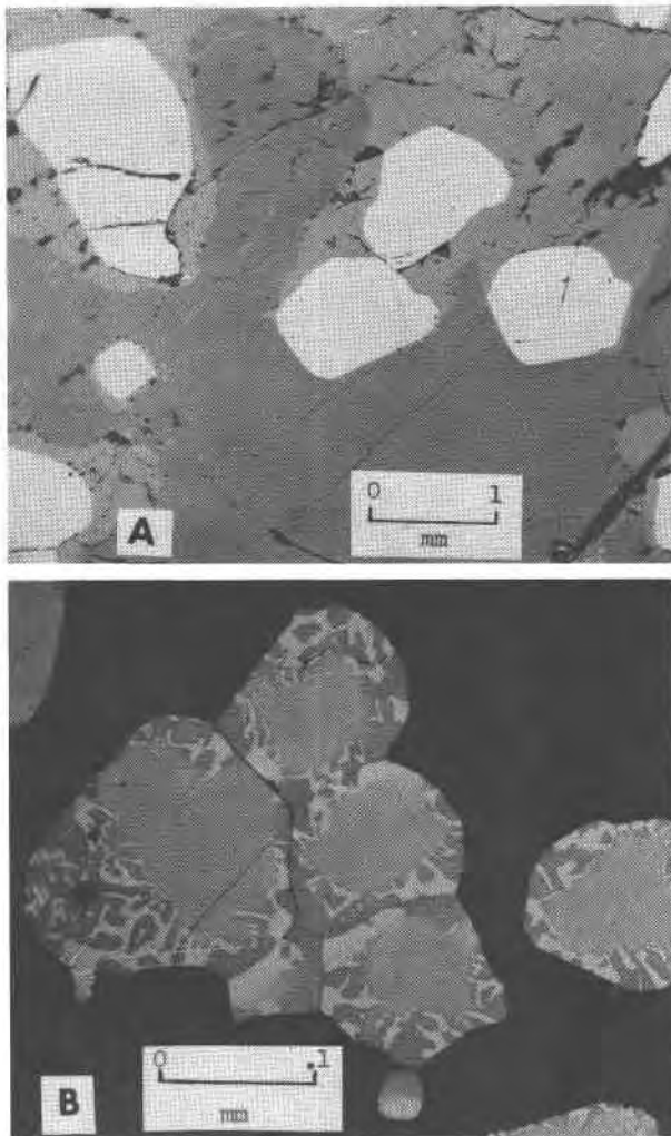
FIG. 3. (a) Euhedral to subhedral crystals of titanian chromite (white) of intermediate composition, probably pseudomorphous after Ti-poor chromite, South Tweefontein. Gray—silicates.
