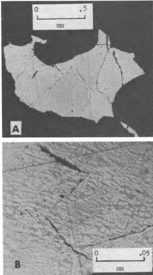
FIG. 4. (a) Magnetite-ulvöspinel anhedral and interstitial to silicates (black), Annex Grootboom.
