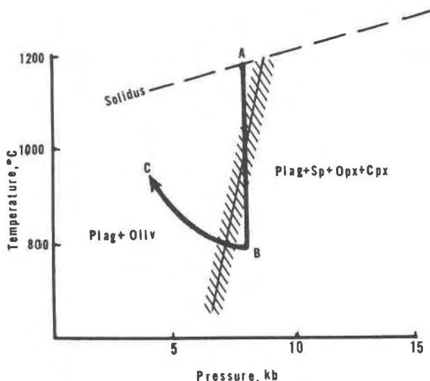
FIG. 3. Diagram of the stability fields of plagioclase, olivine, and spinel in rocks of basaltic composition at high temperatures and pressures. Boundary between the plagioclase + olivine field and that of plagioclase + spinel + pyroxene is taken from Kushiro and Yoder (1966) and Greene and Hibberson (1970) with range of uncertainty indicated by diagonal ruling. Arrow from A to B indicates the postulated cooling of an olivine basalt from its liquidus under isobaric conditions with a resulting reaction of olivine with plagioclase to form spinel and pyroxene with remnant plagioclase. This reaction is reversed during the reheating of the rocks as they rose in the erupting magma (B to C).
