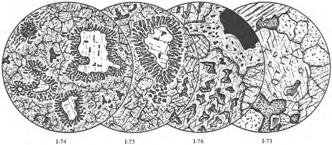
FIG. 1. Textural relations of inclusions. I-74 and I-75 are spinel gabbros with embayed plagioclase (unstippled) surrounded by coronas of spinel (small elongate grains with heavy stippling) and pyroxene (lightly stippled with cleavage). I-76 is a similar rock that has been reheated by its host lava while in transit to the surface. A large nearly opaque grain of spinel in the upper right has partially reacted with the surrounding pyroxene to form a zone of olivine and plagioclase. All of the olivine is now altered to serpentine and magnetite and part of the plagioclase is altered to prehnite. I-73 is a biotite-bearing lherzolite with olivine (upper right), enstatite (top), clinopyroxene (lower right), irregular large grains of brown spinel (heavily stippled), and small flakes of brown biotite.
