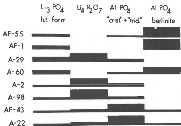
FIG. 4. Heating products of 8 chemically analyzed samples, as determined at room temperature by X-ray powder diffractometry in the products of d.t.a. treatment to 1000°C. Heights of blocks indicate the relative abundances of the individual phases. The tridymite and cristobalite forms of AlPO_4 are always present in about equal amounts.
