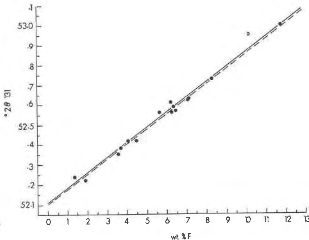
FIG. 6. Measured values of the 2\theta_{CuK\alpha} angles for the 131 reflection plotted against the F contents. The solid line is the regression line calculated for the measured data, the dashed line is that derived from values calculated from unit cell dimensions (see Tables 2 and 3).
