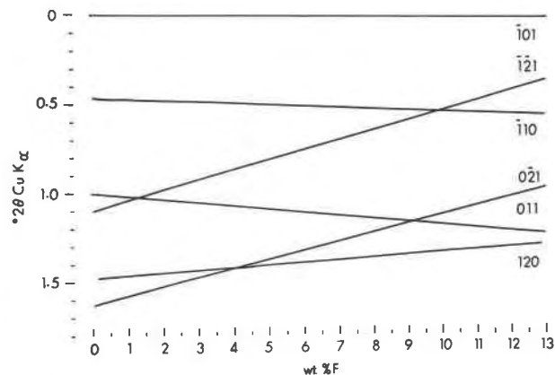
FIG. 7. The variations in angular distances of the X-ray powder diffraction reflections \bar{1}\bar{2}1 , \bar{1}10 , 0\bar{2}1 , 011 , and 120 from the \bar{1}01 reflection. Regression equations are quoted in Table 3.
