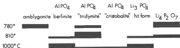
FIG. 5. Heating products of sample A-60 (6.17 wt percent F) as determined by X-ray powder diffractometry at room temperature after each endotherm in d.t.a. treatment. Heights of blocks indicate the relative abundances of the individual phases.
