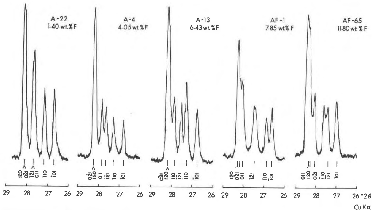
FIG. 8. Typical examples of the group of 6 reflections used for indirect determination of the F content by aid of Figure 7. Note the very good definition of all the \bar{1}01 reflections, used as zero points in reading the angular distances.
