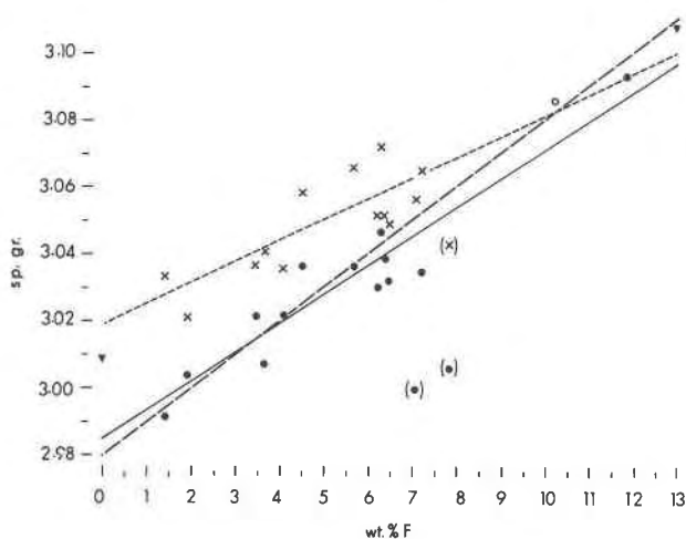
FIG. 1. Specific gravities (measured—dots; calculated—x; theoretical for ideal end members—triangles) plotted against F contents. Points in parentheses were not used in calculations of regression equations. Solid line—regression line for the measured data; heavy broken line—connects the 2.98 and 3.11 values given by Palache et al. (1943) for the end members; light broken line—regression line for the calculated data. Empty circle is the plot of the Na-rich Hebron sample (AF-55).
