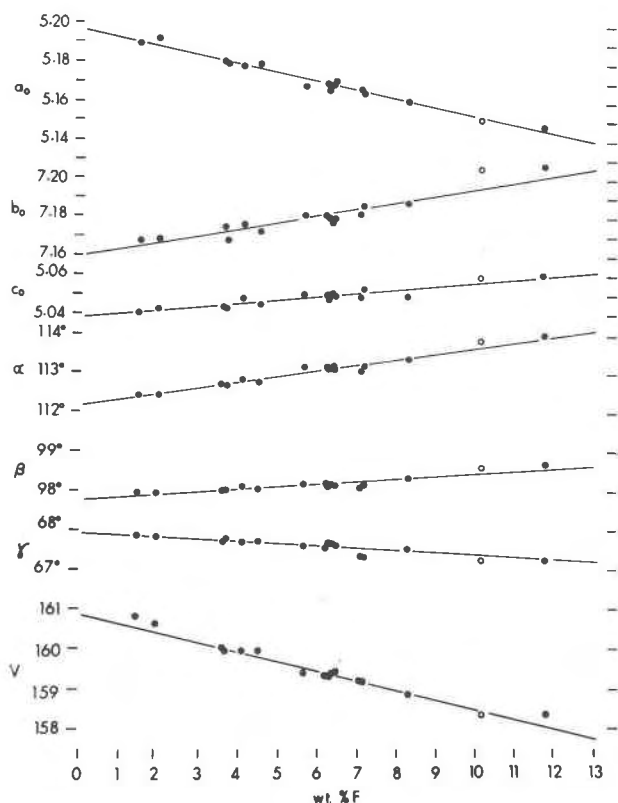
FIG. 9. Unit cell dimensions plotted against the F contents. Regression lines are calculated from equations given in Table 3. Empty circles are the plots of the Na-rich Hebron sample (AF-55).
