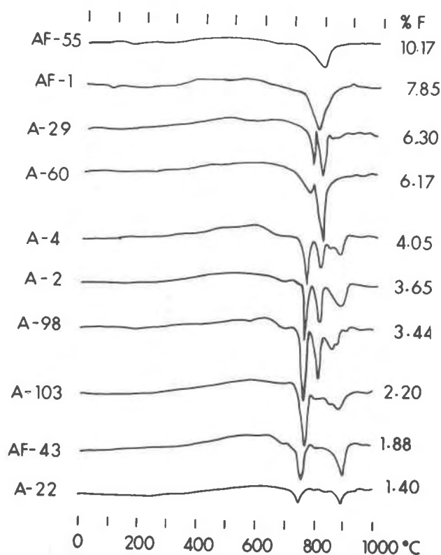
FIG. 3. Differential thermal analysis records of 10 chemically analyzed specimens; weight percentages of F are given at the right-hand side. Temperatures of reaction peaks are listed in Table 4.
