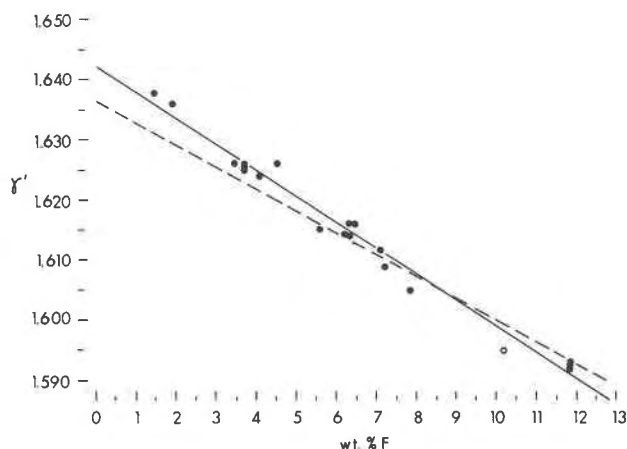
FIG. 2. The refractive indices \gamma' plotted against the F contents. The solid line is the regression line calculated from these data; the broken line is that given by Winchell and Winchell (1951) for true \gamma . Empty circle is the plot of the Na-rich Hebron sample (AF-55).
