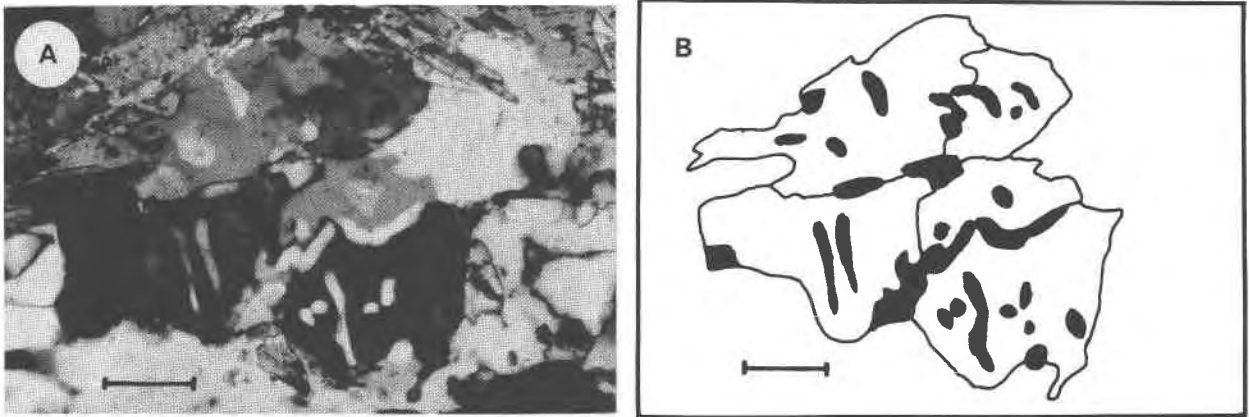
FIG. 6. (A) Five myrmekitic grains in specimen 964 with quartz along the oligoclase grain-boundaries. (B) is a tracing from (A) to show clearly the five grains and the position of the quartz (blacked in).
