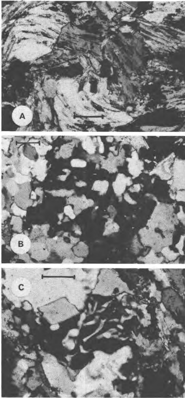
FIG. 2. Three varieties of inclusions in the Haast Schist oligoclases. Scale marks represent 0.1 mm. (A) Opaque minerals and biotite trails in specimen 961. (B) Centered in photograph from specimen 964 is an almost extinct plagioclase approximately 0.5 \times 0.3 mm with very fine twin-lamellae visible running across but slightly down towards the right of the grain. The plagioclase includes irregular quartz blebs (not extinguished) and mosaics which merge outwards with the surrounding quartz mosaic. The tiny bright specks in the plagioclase are mainly sericite inclusions. (C) Rods of quartz branching towards the top right corner in the extinguished oligoclase grain at center of photograph from specimen 962.
