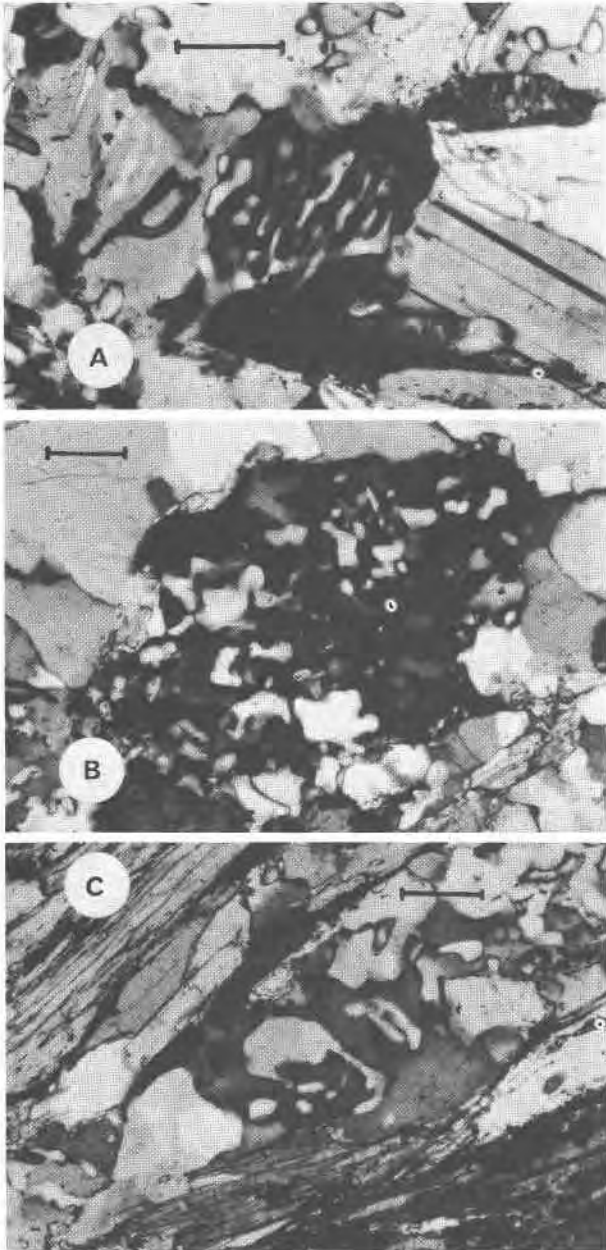
FIG. 3. Textures observed in specimen 963, each scale mark representing 0.1 mm. (A) Myrmekite with quartz rods branching, then joining together again at center of photograph. (B) Several groups of sub-vermicular quartz grains in one oligoclase crystal (in extinction). This is an intermediate stage between textures shown in Figure 2B and 2C. (C) Centered in photograph is a quartz bleb grading outwards into quartz rods within an (almost extinct) oligoclase crystal.
