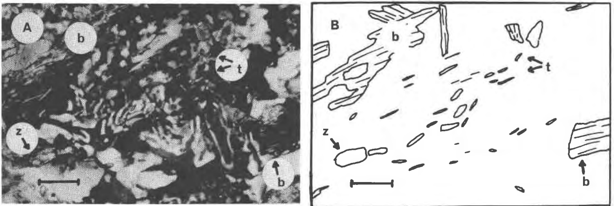
FIG. 5. (A) Myrmekitic plagioclase in specimen 966 with most quartz rods branching upwards and slightly to the left. Trails of biotite and clinozoisite within the myrmekite are just visible on the photograph (t) and are represented for clarity on the tracing (B). Other grains of biotite (b) and clinozoisite (z) at the boundary of the myrmekite are also shown. Scale mark represents 0.1 mm.
