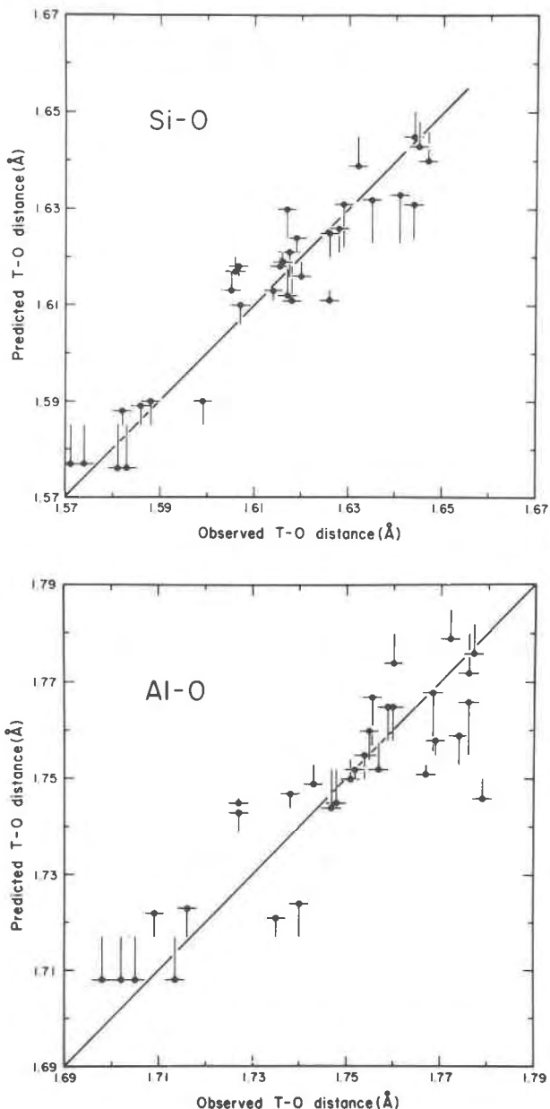
FIG. 2. Graphs of the observed Si-O and Al-O distances against those calculated using the variables \Sigma Ca^2 and -1/\cos(T-O-T') . The dots represent the values obtained using both variables, while the ends of the vertical lines opposite them represent the values predicted by \Sigma Ca^2 alone. The horizontal lines represent the standard errors in the observed distances reported by Wainwright and Starkey (1971). The equations used to calculate the distances are:
