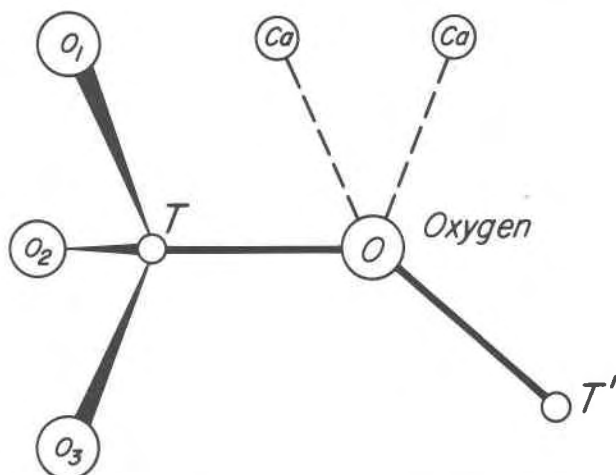
FIG. 1. A schematic representation of a portion of the anorthite structure. The distance T-O is considered as the dependent variable. The independent variables considered are listed in Table 2.
