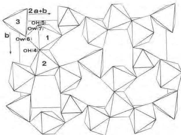
FIG. 4. Projection of Na-octahedra in tincalconite on (001).
