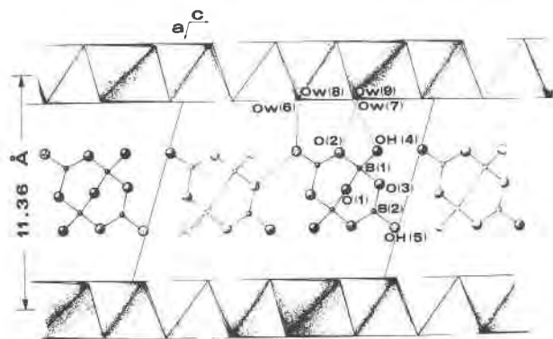
FIG. 3. The structure of borax projected on (010). Some of the hydrogen bonds are shown by dotted lines (Morimoto, 1956).
