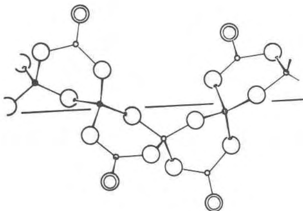
FIG. 6. Boron-oxygen chain running along the bisector of monoclinic angle in kernite (Cialdi et al. , 1967).
