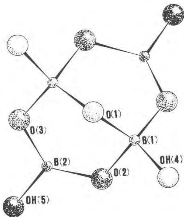
FIG. 2. [B_4O_5(OH)_4]^{2-} polyanion in tincalconite.
