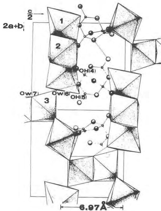
FIG. 1. Projection of tincalconite structure on (010) of the orthohexagonal cell. Dotted lines indicate some of the hydrogen bonds.
