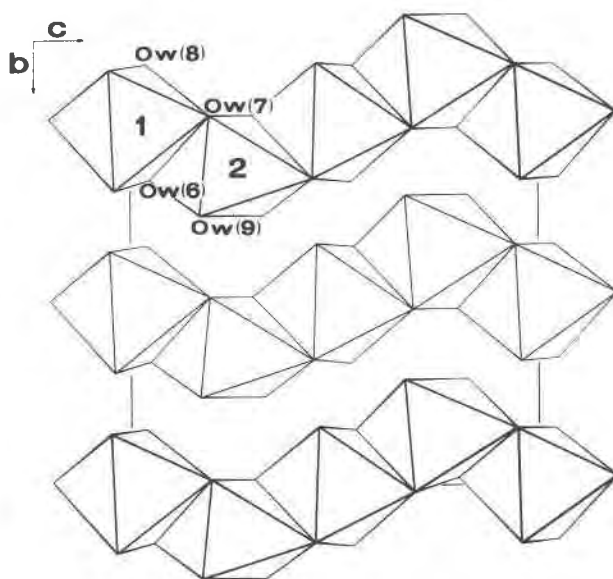
FIG. 5. Projection of Na-octahedra in borax on (100) (Morimoto, 1956).
