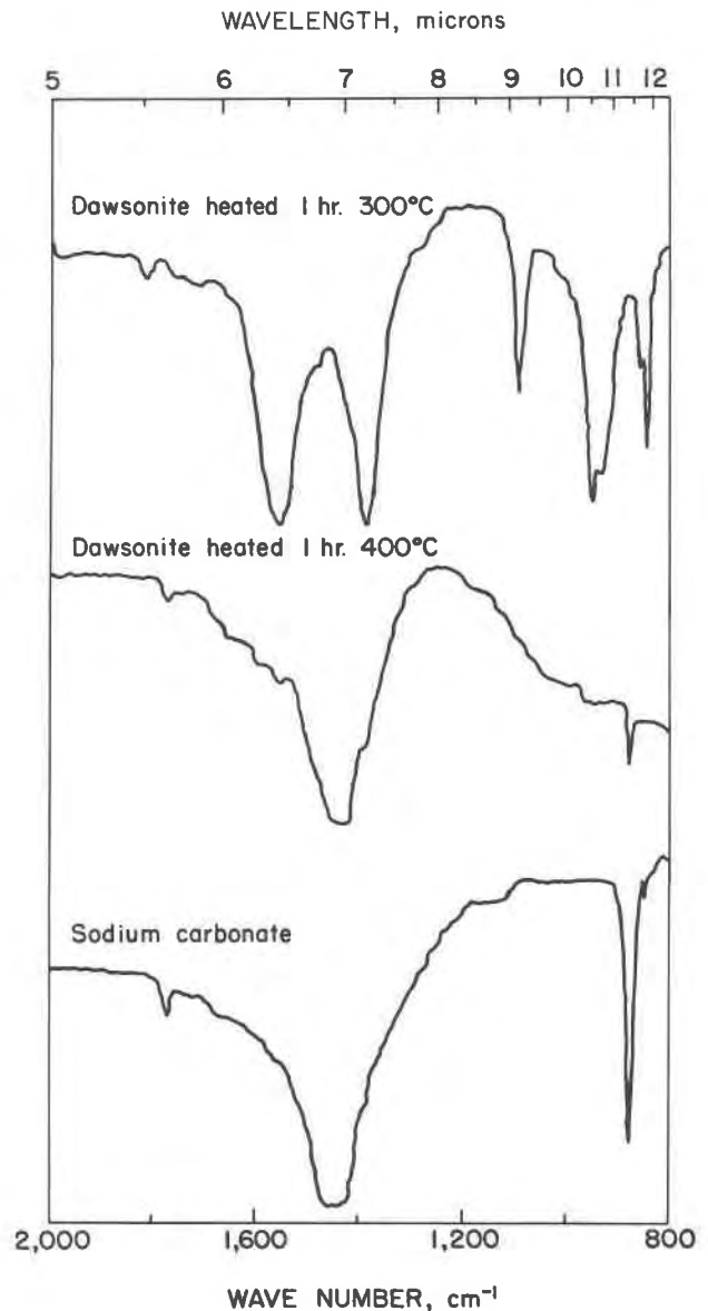
FIG. 2. Infrared spectra of heat treated dawsonite and sodium carbonate.
